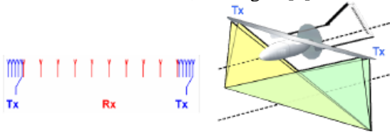
Fig.2. Antenna concept of a thinned antenna array with a set of transmitters (Tx) and receiver antenna elements (Rx) mounted along the wings.
