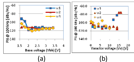
Fig. 1 Phase noise of 5 GHz balanced Colpitts oscillators (a) fixed-frequency vs base voltage (b) phase noise of VCO vs varactor voltage.
