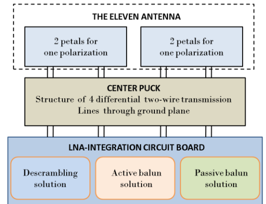
Figure 1 System configuration of the Eleven feed
