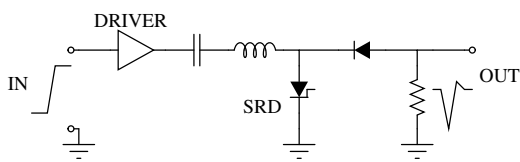
Figure 1: SRD pulse generator diagram.
