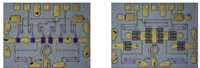
Fig. 2. SPDT-1 (left) and SPDT-2 (right). Chip dimensions are 1.4 \times 1.1 \text{ mm}^2 and 1.5 \times 1.1 \text{ mm}^2 respectively.
