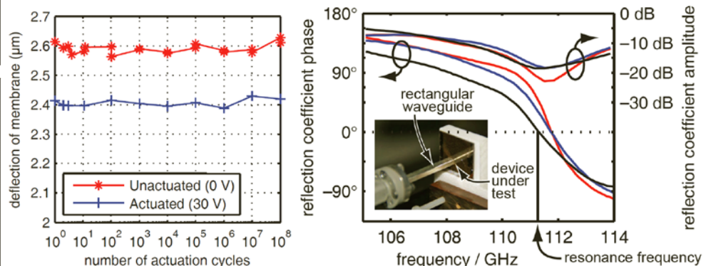
Fig. 3: Life-cycle measurement to over 100 million actuation cycles.
