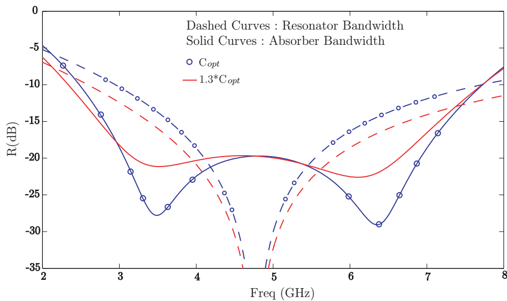
Figure 3: Comparison of the series RLC resonator bandwidth (equivalent to FSS structure it models) and the corresponding single layer circuit analog absorber.
