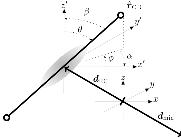
Figure 2: An antenna current distribution is depicted as a tilted ellipsoid, positioned at the radiation center \mathbf{d}_{\text{RC}} and with major axis along the current distribution axis \hat{\mathbf{r}}_{\text{CD}} . The current distribution axis is indicated as a line ended by two circles. Two parallel coordinate systems are shown: the far field reference system xyz , and a parallel x'y'z' system with origin at \mathbf{d}_{\text{RC}} . The coordinate translation \mathbf{d}_{\text{min}} = -\mathbf{d}_{\text{RC}} leading to minimum L^2 results in a centered antenna current (the ellipse) in the xyz system. A subsequent minimization of L_z^2 yields a rotation that aligns the antenna current (the ellipse) to the z -axis. This rotation can be decomposed in a first rotation \alpha = -\phi around the \hat{\mathbf{z}} -axis, and a secondary rotation \beta = -\theta around the y -axis.
