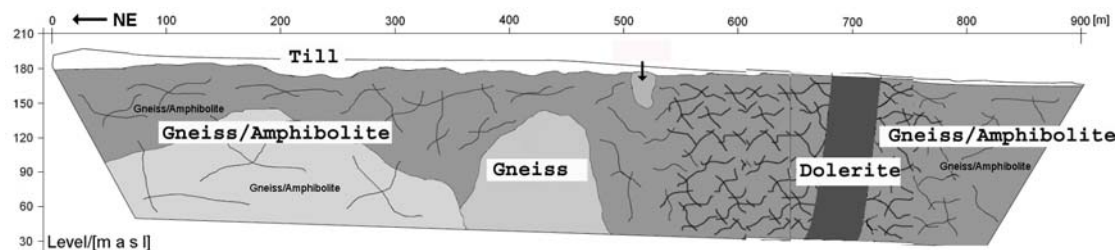
Figure 3. Detailed geological interpretation of the 900 metre profile.
