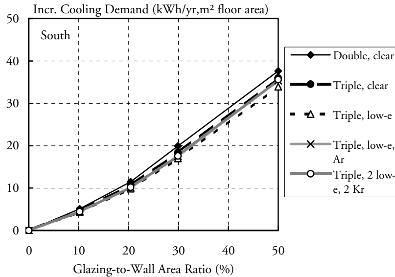
Figure 5.24 Incremental cooling demand (kWh/yr, m² floor area) as a function of GVAR and window type for a south facing office in Lund
