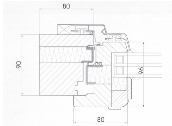
Figure 3.15 Two examples of German windows with total window U -values around 0.7 \text{ W/m}^2\text{K} .
