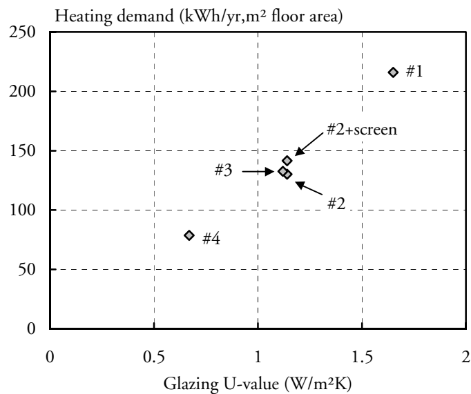
Figure 5.31 Annual heating demand (kWh/yr, m 2 floor area) as a function of glazing U-value.
