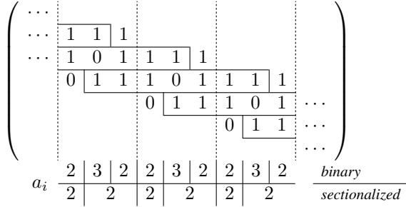
Fig. 5. Number of active rows a_i for the rate R = 2/3 convolutional code H_{eq} = (1 + D + D^2 \ 1 + D + D^2) , before (upper row) and after sectionalizing (lower row). The boxes surround the active part of each row.
