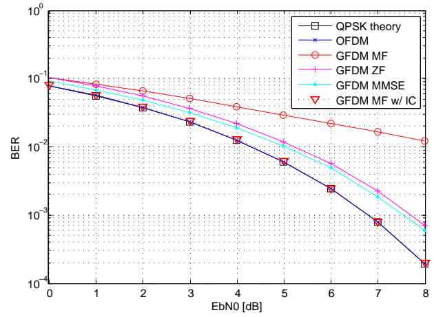
(b) K = 128, M = 5, \alpha = 0.5
