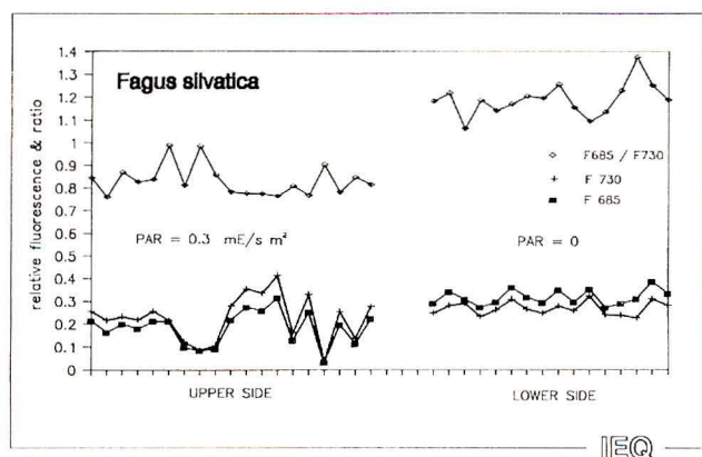
Fig. 9 - Point monitoring of upper and lower sides of beech leaves using the CNR-IEQ two-channel fluorosensor. Individual channel intensities and the ratio of the two channel readings are plotted.
