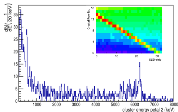
Figure 2: \gamma -ray energy spectrum following (p,2p) reactions on the water target. The 6.3-MeV transition in 15 N is clearly visible. The inset shows the proton tracking data from a DSSSD-petal pair used in the event selection cut.
