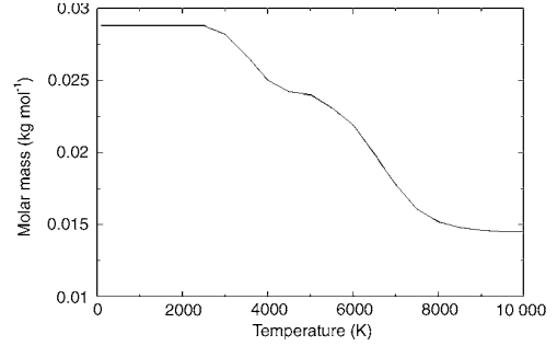
Figure A2. The molar mass of air as a function of the temperature.
