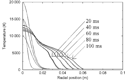
Figure 5. Temperature profiles for four different choices of initial profiles of the temperature ( T_{max0} = 20 kK, a = 10 mm; T_{max0} = 15 kK, a = 10 mm; T_{max0} = 10 kK, a = 10 mm; T_{max0} = 15 kK, a = 5 mm) at a current I = 500 A. The differences in the initial profiles have minor effect on the later profiles.
