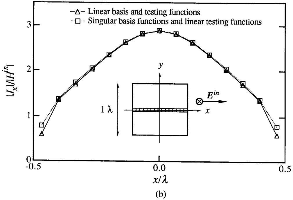
Fig. 14. The current density parallel to the incident electric field, i.e., J_x . The mean values of the current density on the sub-squares in the middle row parallel to the direction of the current are shown, i.e., along the x -axis. The length of the side of the plate is (a) 0.5\lambda and (b) 1\lambda . In both cases the plate is divided into 15 \times 15 sub-squares.
