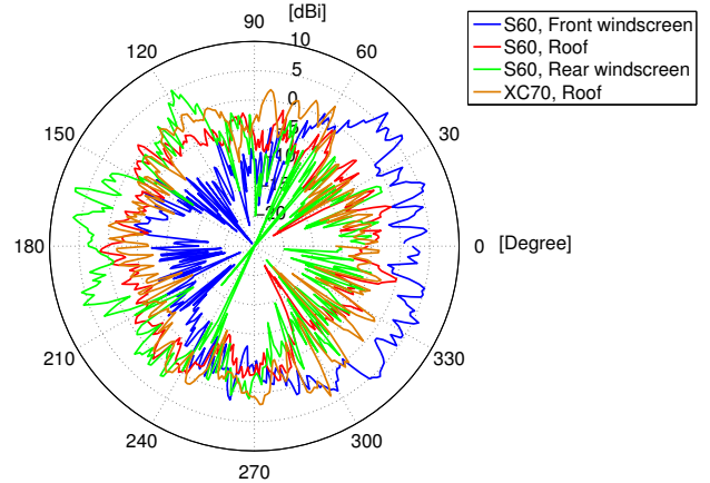
Fig. 3. Measured antenna pattern, mounted on the Volvo S60 and the Volvo XC70. The front of the cars is at 0^\circ . The antenna pattern of the V70 and XC90 is similar as the presented XC70 since all these models have similar design of the roof area.
