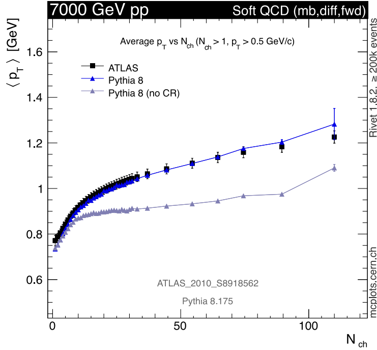
Figure 1: \langle p_{\perp} \rangle(n_{ch}) with the default PYTHIA 8 Tune 4C [21], and the same with CR switched off, compared with ATLAS data [22].
