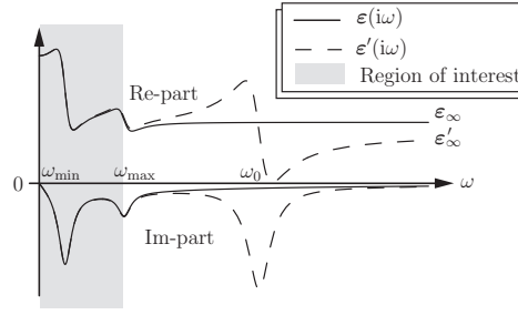
Figure 3: Illustration of the approximation of the constitutive relations. The original constitutive map \epsilon(i\omega) with the instantaneous response \epsilon_\infty is approximated by the constitutive map \epsilon'(i\omega) with the instantaneous response \epsilon'_\infty < \epsilon_\infty . The error of the approximation approaches zero in the region of interest [0, \omega_{\max}] as the approximation parameter \omega_0 \rightarrow \infty .
