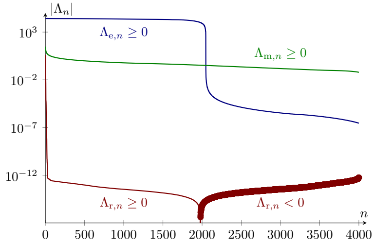
Figure 28: Eigenvalues \Lambda_n of \mathbf{X}_e , \mathbf{X}_m , \mathbf{R} for a planar rectangle with side lengths \ell_x = 2\ell_y = 0.1\lambda divided into 64 \times 32 elements (4000 basis functions).
