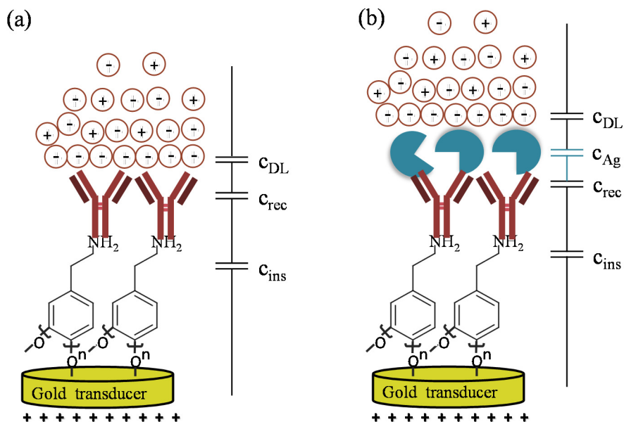
Fig 4.6: Schematic representation of a capacitive surface showing (a) contribution of capacitance by different layers of a modified gold electrode and (b) additional layer introduced upon analyte binding.
