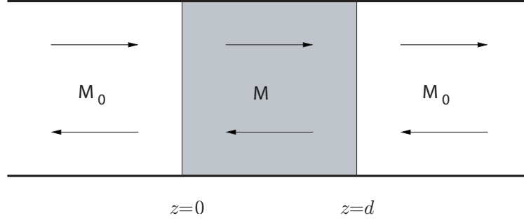
Figure 2: The scattering geometry in the waveguide. The material under test (MUT) is confined to the region 0 < z < d with material parameters \mathbf{M} , and the surrounding parts of the waveguide are filled with material \mathbf{M}_0 , usually air.
