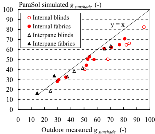
Figure 5.1 Comparison between outdoor measured and ParaSol simulated g_{\text{sunshade}} for interpane and internal products.
