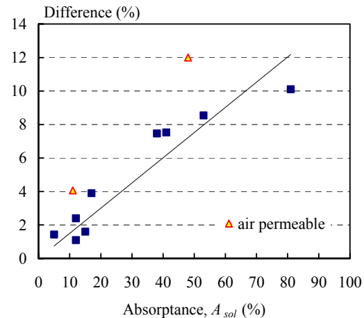
Figure 5.2 Difference between outdoor measured and ParaSol simulated g_{\text{sunshade}} vs the material absorptance for internally mounted fabrics + a linear fit.
