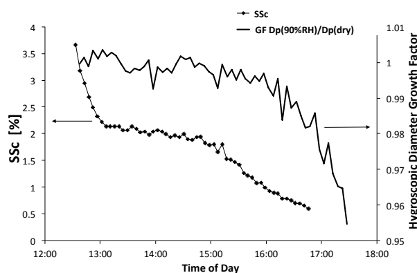
Figure 1. Preliminary SS_c decline for diesel soot particles ( d_{dry}=150 nm) (data points), as well as the corresponding GF at 90% RH (solid black line) over time.
