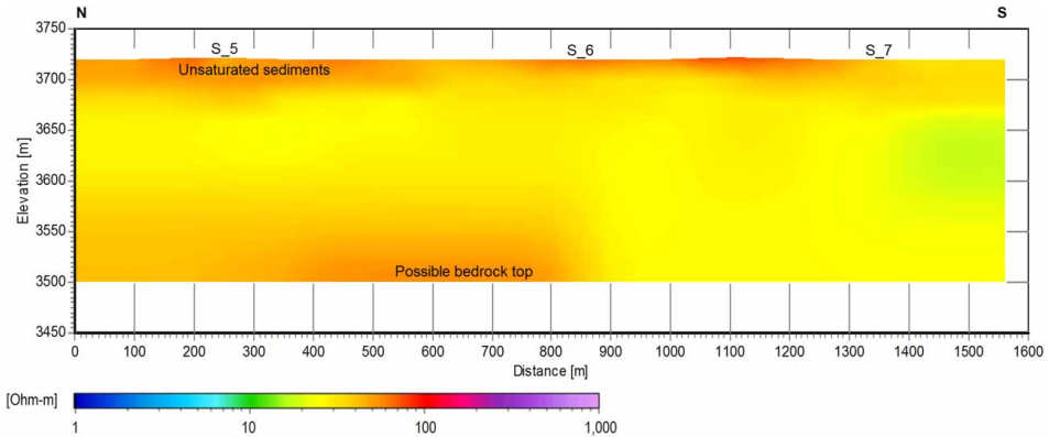
Figure 5 | 2-D resistivity model corresponding to the ERT line C. Unsaturated sediments characterized by relatively high resistivity can be seen at shallow parts of the section.
