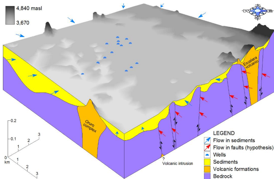
Figure 7 Hydrogeological conceptual model in the central part of the alluvial fan.
