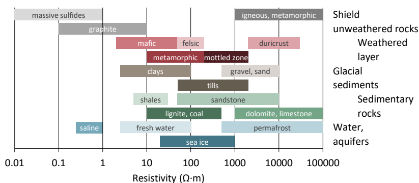
Figure 10 Typical resistivity and conductivity ranges for geological materials. Modified from Palacký (1987).
