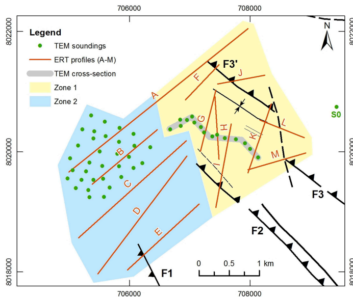
Fig. 4. Location of the TEM and ERT measurements. Data are divided and shown later in two separated zones (black marks are faults and structures, same as in Fig. 2a).
