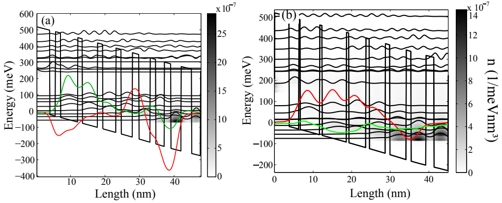
Figure 5.5: Carrier density and spatially resolved gain (a. u. ) at a current density of 4 kA/cm 2 , at (a) \hbar\omega = 100 \text{ meV} (red) and \hbar\omega = 160 \text{ meV} (green) of the 7.3 \mu\text{m} structure, and at (b) \hbar\omega = 105 \text{ meV} (red) and \hbar\omega = 140 \text{ meV} (green) of the 12 \mu\text{m} structure.
