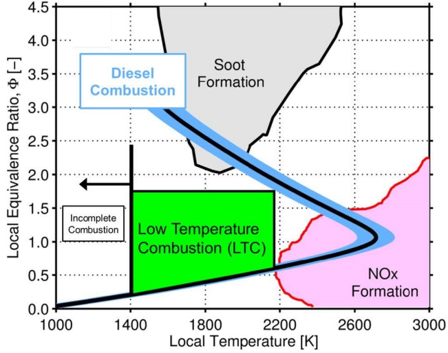
Figure 2.6: Regions of \text{NO}_x and soot formation in local equivalence ratio ( \Phi ) versus local temperature space [23], \text{NO}_x and soot islands calculated from n-heptane chemical kinetic simulations [18].
