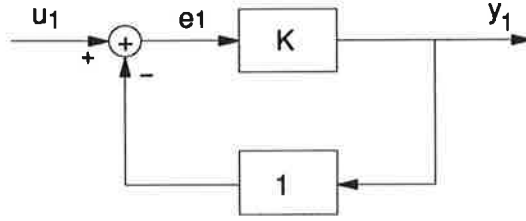
Figure 2. The feedback system of Example 1.
