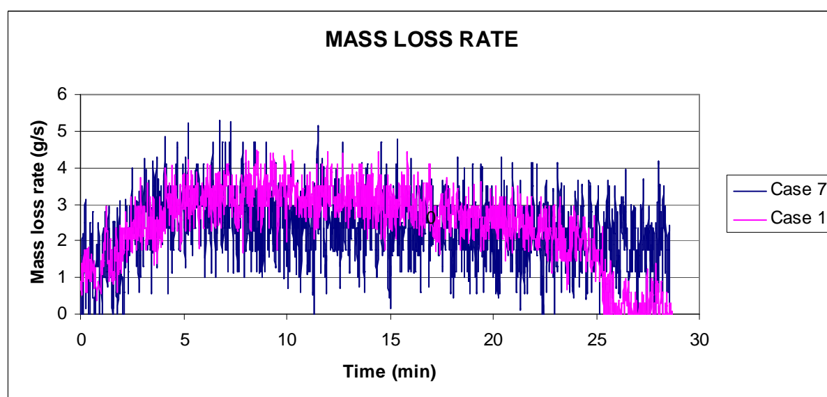
Diagram 8.2: Mass loss rate for test 1 and test 7.
