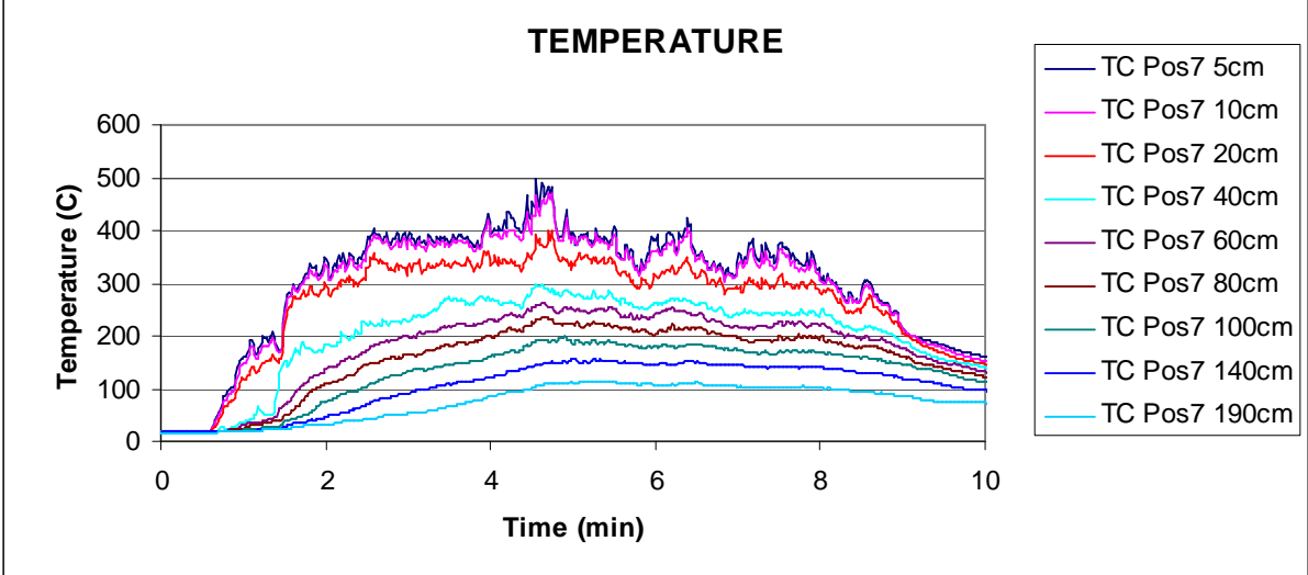
Diagram O 2: Temperature profiles
