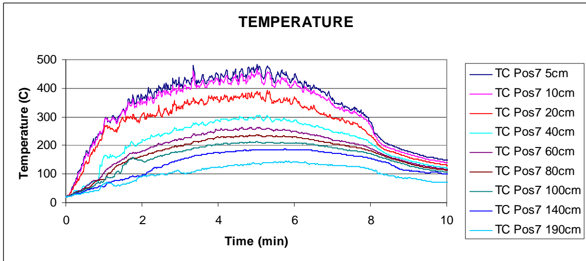
Diagram 8.7: Test 10 with the fuel area 650 \times 650 mm.
