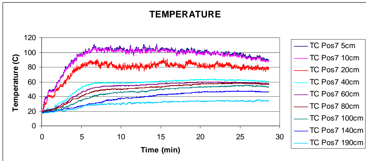
Diagram R 2 Temperature profiles
