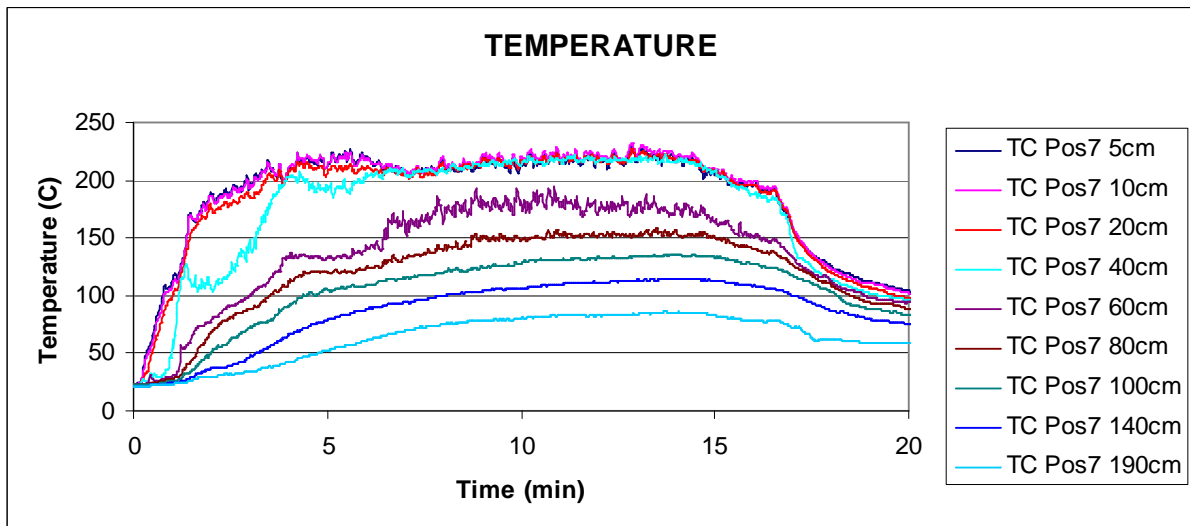
Diagram Q 2: Temperature profiles.
