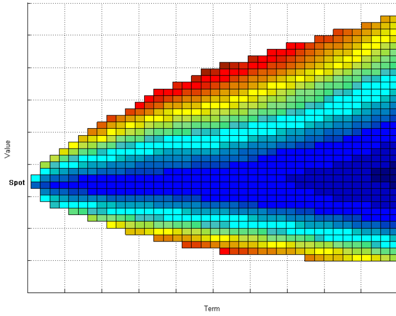
Figure 16: The Local volatility surface as a function S_t and t of seen from above.
