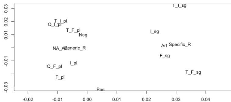
Figure 4. Interaction of Axiology, Article, Collocation and Referent Type.
