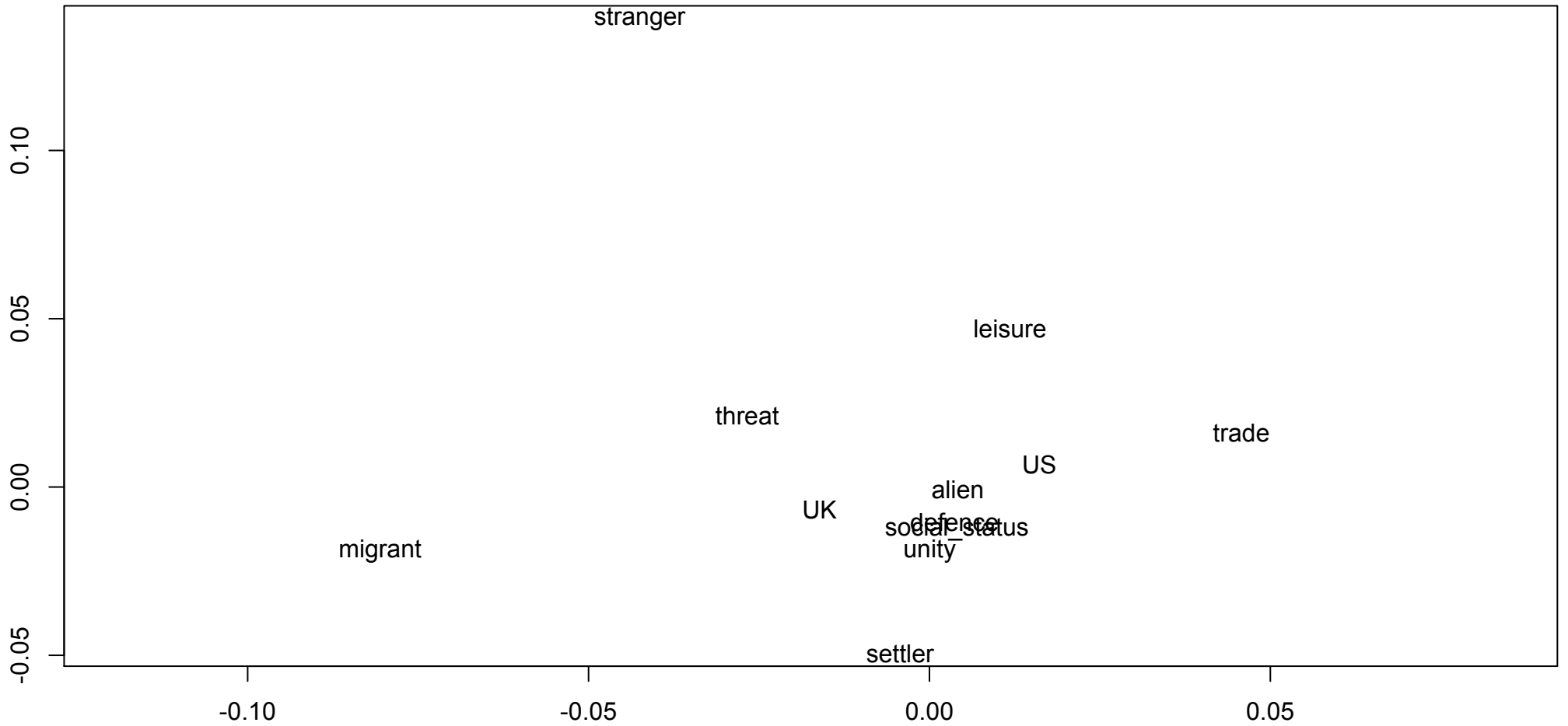
Figure 10. Interaction of Dialect, Dictionary and Theme Coarse. Multiple Correspondance Analysis.
