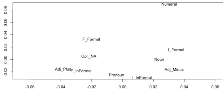
Figure 2. Interaction of Style - Lexeme and Class Collocation. Multiple Correspondence Analysis.
