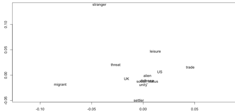
Figure 10. Interaction of Dialect, Dictionary and Theme Coarse. Multiple Correspondence Analysis
