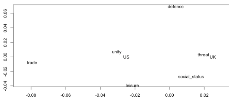
Figure 8. Interaction of Theme Coarse and Dialect. Multiple Correspondence Analysis
