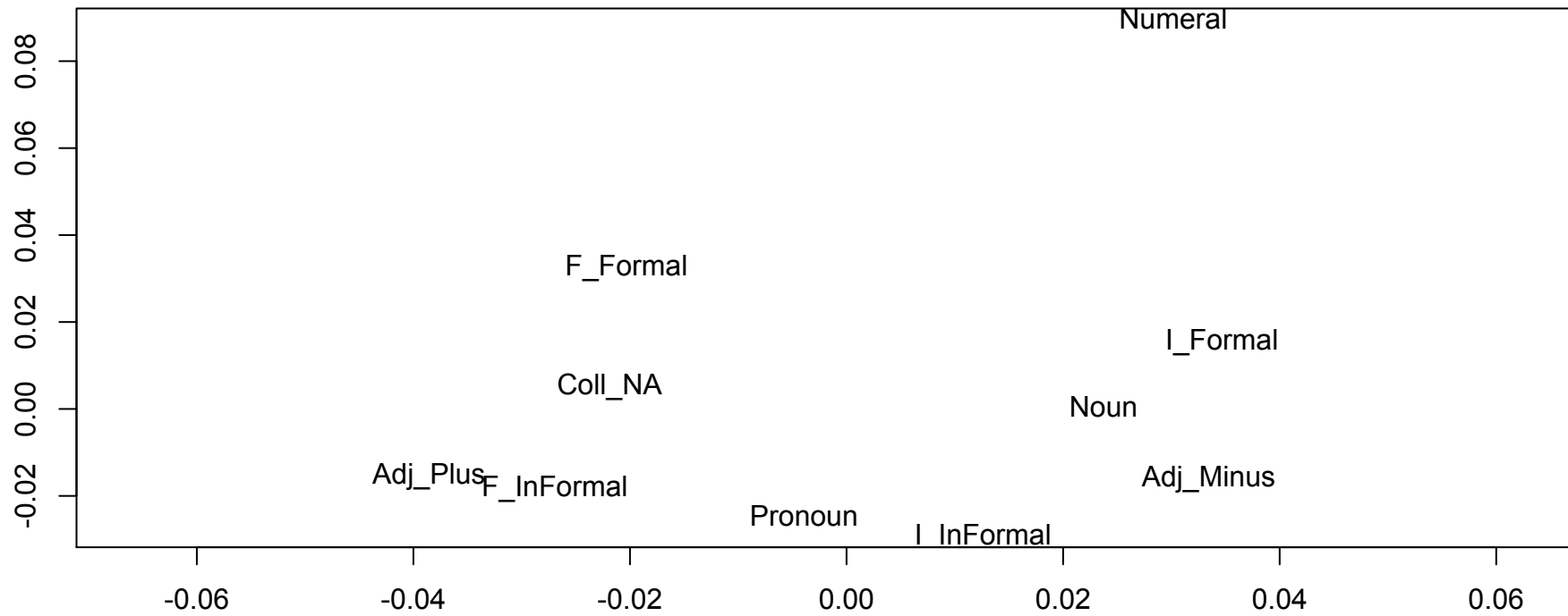
Figure 2. Interaction of Style - Lexeme and Class Collocation. Multiple Correspondance Analysis.
