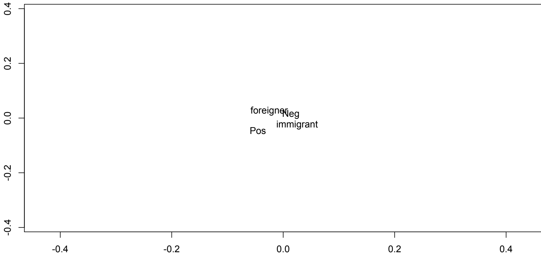
Figure 1. Interaction of Lexeme and Axiology. Multiple Correspondance Analysis ( The MCA)
