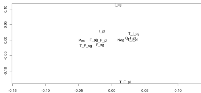
Figure 3. Interaction of Collocation and Axiology. Multiple Correspondence Analysis
