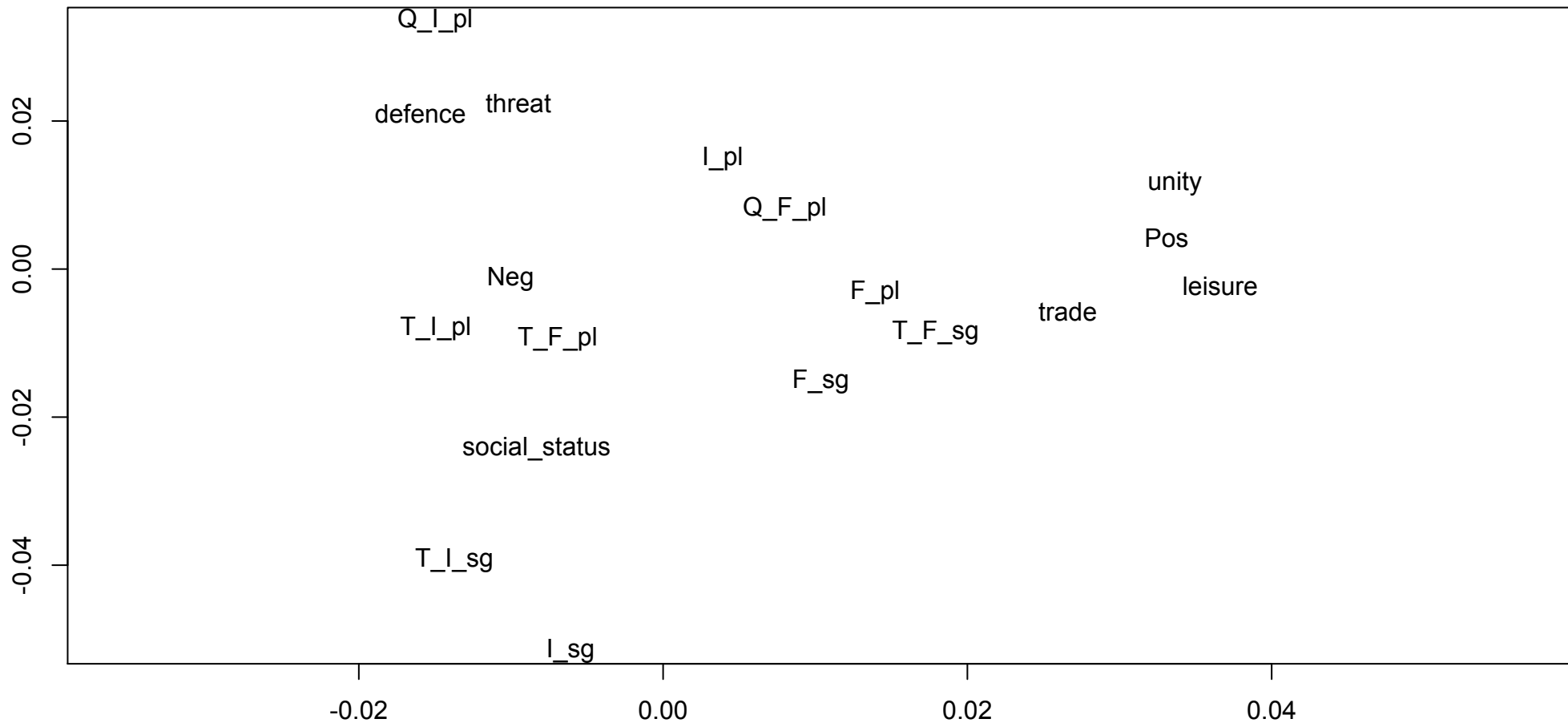
Figure 6. Interaction of Axiology, Collocation and Theme Coarse. Multiple Corrsepondence Analysis
