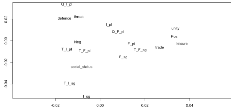
Figure 6. Interaction of Axiology, Collocation and Theme Coarse. Multiple Correspondence Analysis
