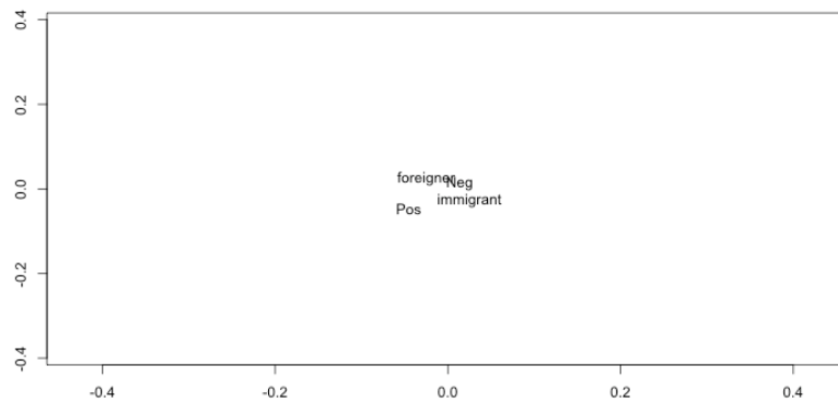
Figure 1. Interaction of Lexeme and Axiology. Multiple Correspondence Analysis (MCA)
