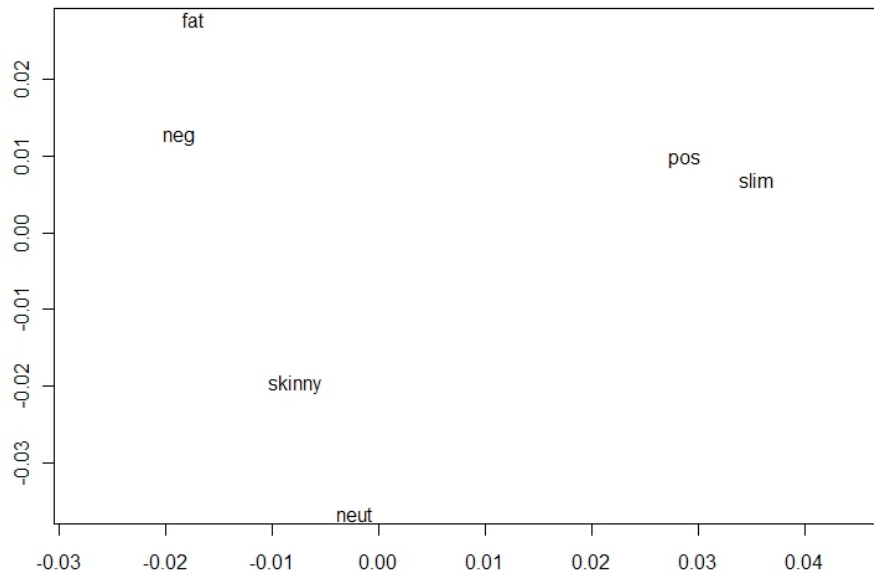
Figure 1. Interaction of Axiology and Lexeme. Correspondence Analysis.
