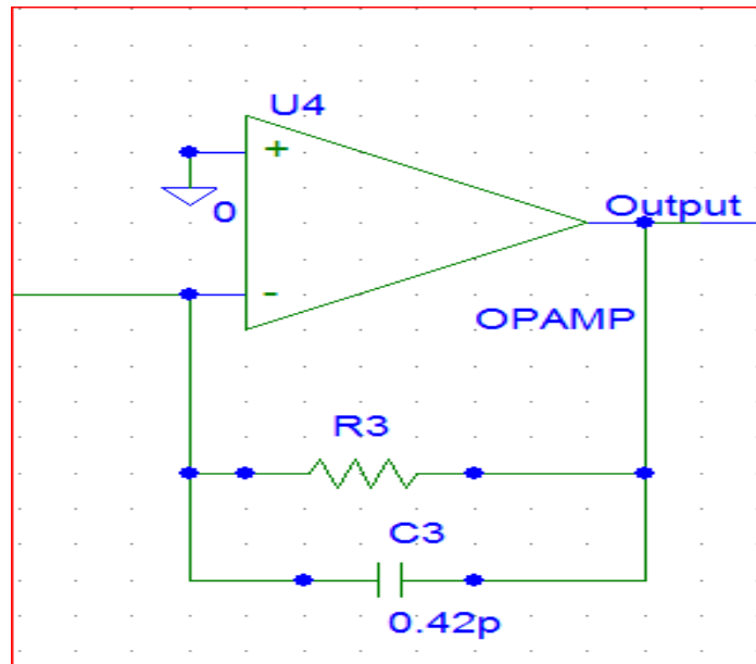
Figure 6.3 CSA schematic circuit
