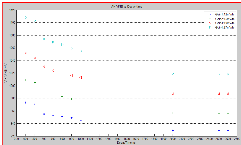
Figure 6.13 DC level differences versus preamp decay time with different gains (Other configurations: Polarity 1, preamp disabled, peaking time 120 ns)
