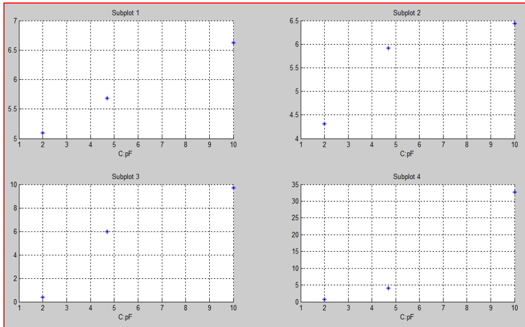
Figure 6.17 ADC error of various gains versus additional input capacitance (i.e. in addition to the amplifier input capacitance)
