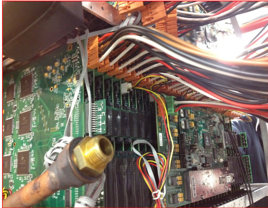
Figure 4.8 FECs fully connected with RCU and LV-power
