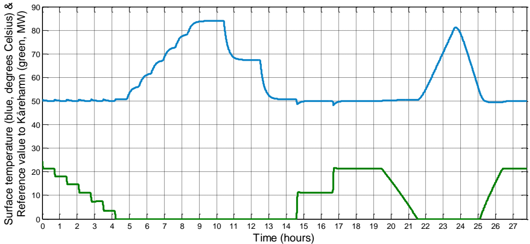
Figure 5-13. Result of simulation, for varying ambient temperature at conductor, with 0 m/s wind speed and varying wind direction. The blue signal shows the surface temperature of the conductor in °C, the green the reference value to Kårehamn in MW.
