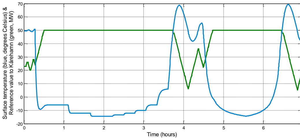
Figure 6-5. Result of simulation, for varying wind speed at conductor, with 90 degrees wind direction and -20 °C ambient temperature. The blue signal shows the surface temperature of the conductor in °C, the green the reference value to Kårehamn in MW.
