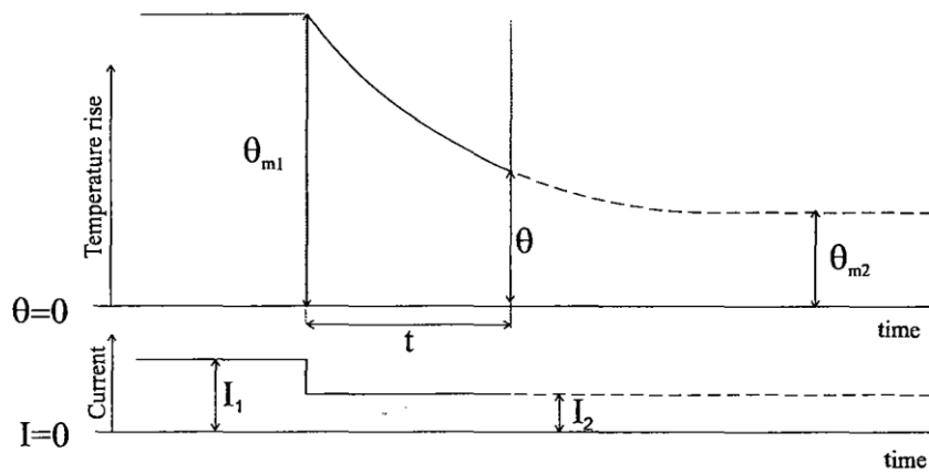
Figure 2-2. [5] Temperature behaviour of an overhead conductor after a decrease in current.
