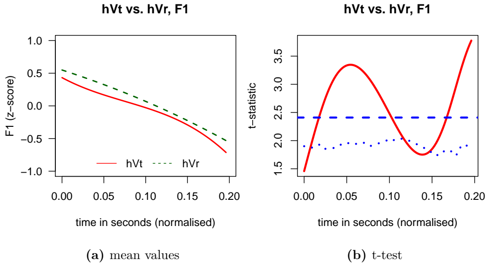
Figure 7 – Average F_1 frequencies in hVr and hVt; (a): means over all speakers; (b): observed statistic (solid red line), critical value (0.05) for the pointwise comparison (dotted line) and maximum of the t-statistics (dashed line)
