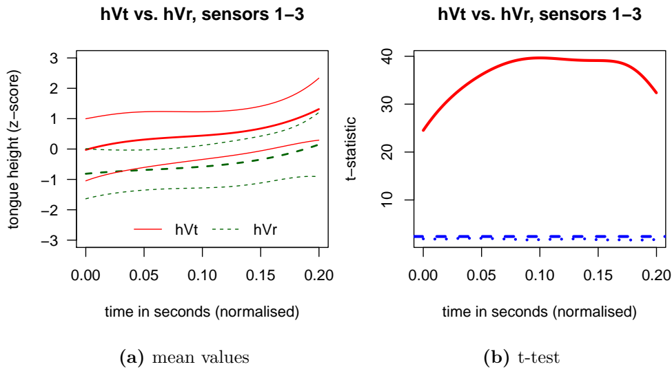
Figure 3 – Comparison of average tongue heights between the pre-r and pre-t allophones of / \epsilon :/ and / \ø :/ (averaged across all 3 sensors and both vowels); (a) : mean values and standard deviations; (b) : observed statistic (upper solid line), critical value (0.05) for the pointwise comparison (lower dotted line) and maximum of the t-statistics (middle dashed line)
