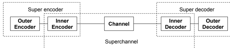
Figure 3.1: Concatenated system
