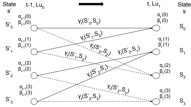
Figure 2.9: Trellis computation of soft output
