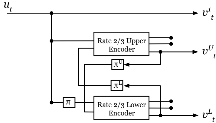
Figure 3.8: BCC encoder
