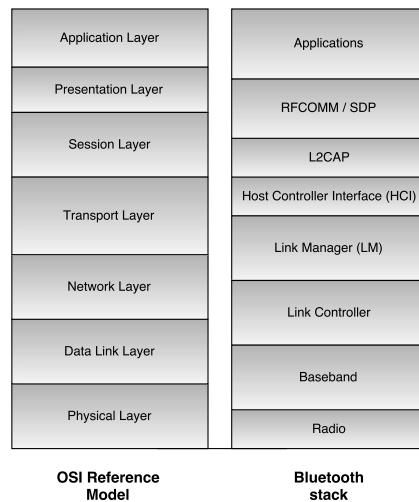
Figure 2.2.: OSI reference model and Bluetooth stack.
