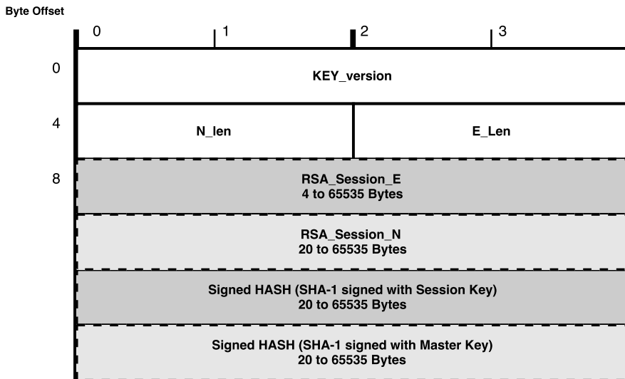
Figure 3.3.: Structure of a theoretical Authentication data packet
