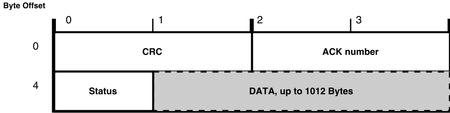
Figure 3.2.: Image of the FOTA header
