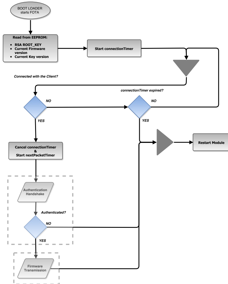
Figure 4.2.: A flow chart diagram of FOTA.
