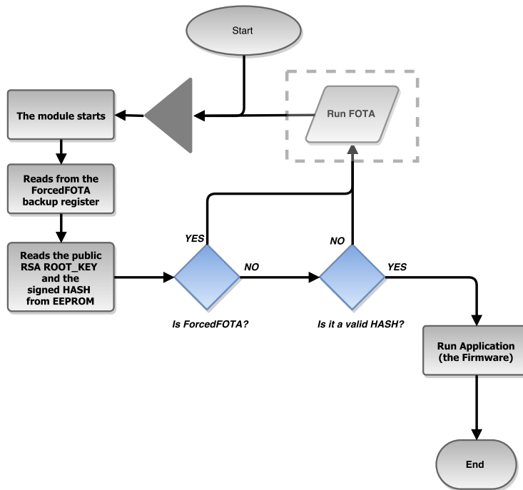
Figure 4.1.: A flow chart diagram of the bootloader.
