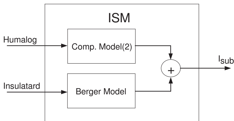
Figure 5.2: The Insulin Sub-Model(ISM).
