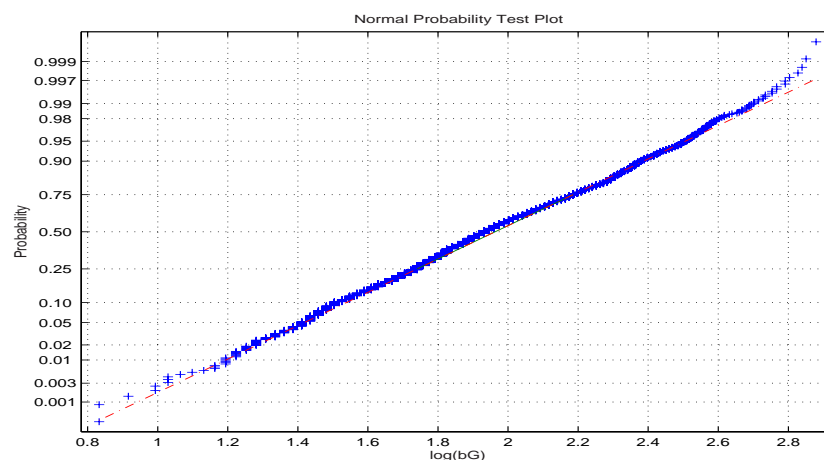
Figure 4.13: Test of log-normality.
