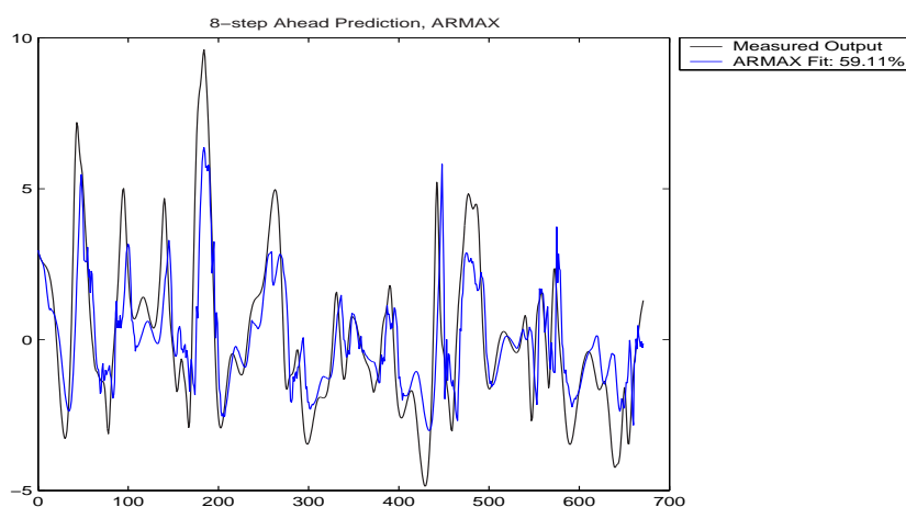
Figure 6.10: 8-step ahead prediction, ARMAX.
