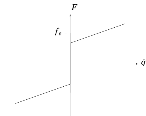
Figure 6.16 Friction model considering stiction, viscous and Coulomb components.
