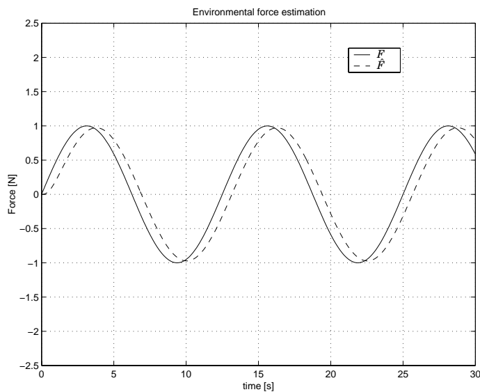
Figure 2.5 Force estimation in presence of a sinusoidal environmental force. The force estimation error is also a sinusoidal which amplitude and phase lag could have been determined a priori from the bode plots of \mathcal{H}(s) (figure 2.1)
