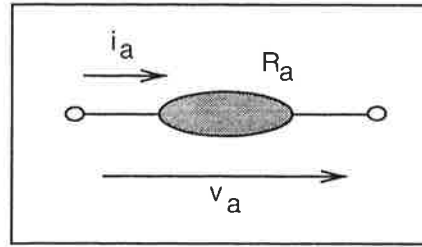
Figure 3.9 The electrical arc as a circuit element
