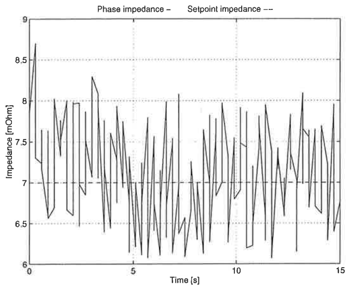
Figure 6.11 The controlled phase impedances for a random disturbance
