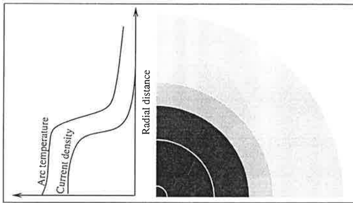
Figure 3.7 Radial current density and temperature distribution in the arc
