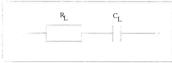
Figure A.1 The electric arc modeled as a capacitive load
