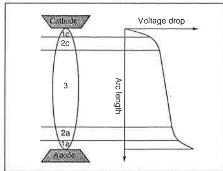
Figure 3.1 The potential distribution in an electric arc
