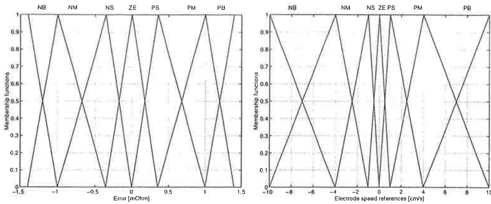
Figure 6.4 The membership functions for the error and speed references
