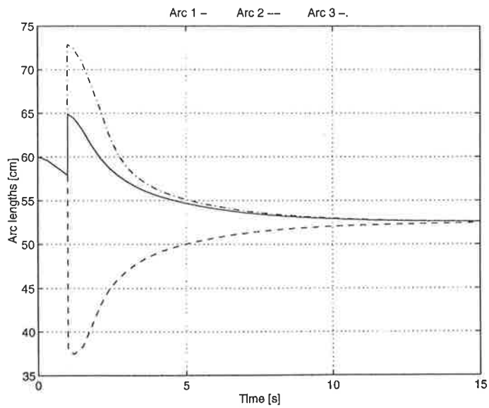
Figure 6.10 The arc lengths for a step disturbance
