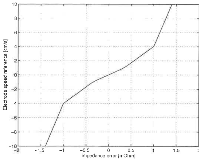
Figure 6.3 The proportional gain nonlinearity
