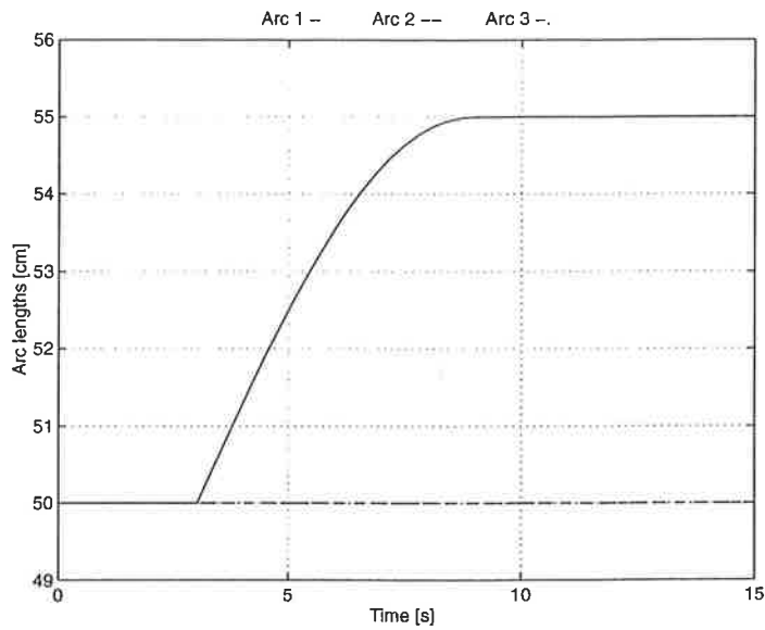
Figure 5.25 The arc lengths when lifting electrode 1
