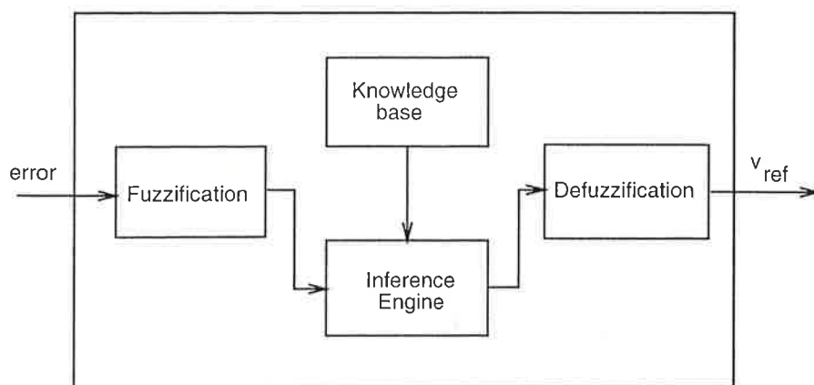
Figure 6.2 The fuzzy logic controller system
