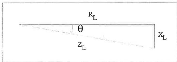
Figure A.2 The arc phase
