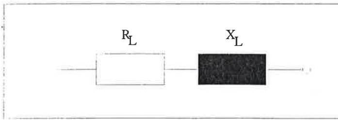
Figure 3.11 Köhle's model of the arc
