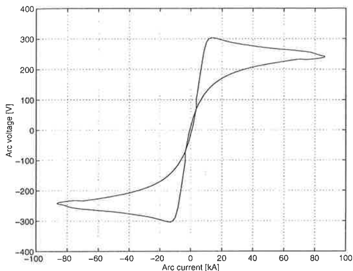
Figure 5.5 The dynamic arc current-voltage characteristic
