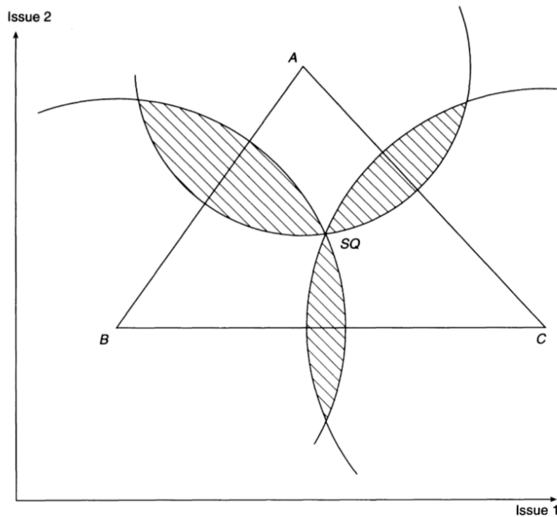
Fig. 1. Winset of status quo with three players in two dimensions
