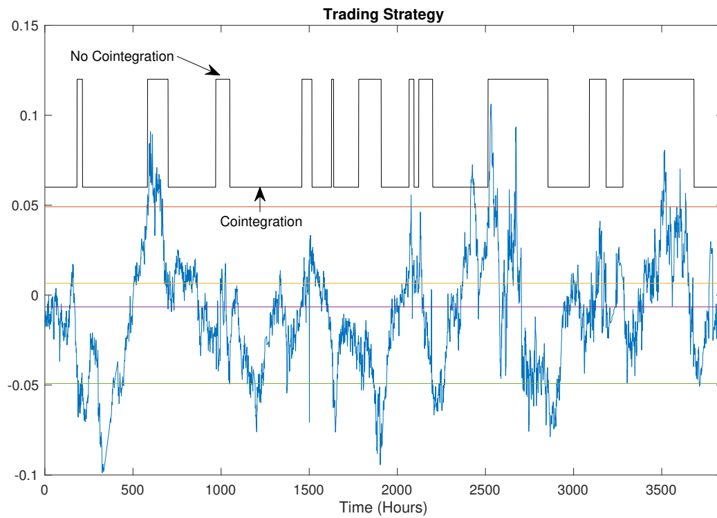
Figure 2.2: Illustration of the trading strategy, showing the regimes, residuals and trading thresholds k_1 - k_4 as horizontal lines.
