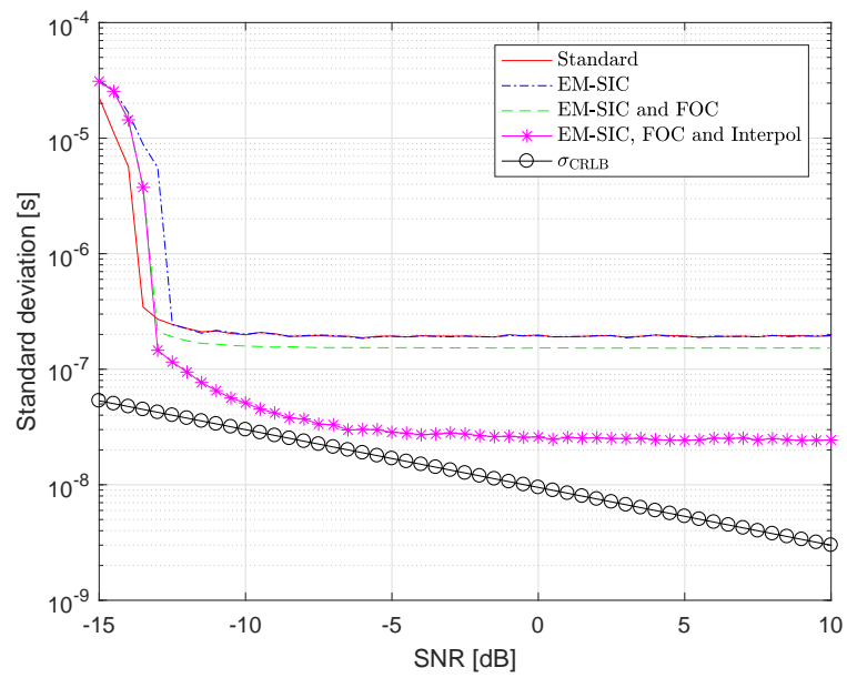
Figure 5.17: Standard deviation of the TOA estimates in AWGN compared to the CRLB for different SNR.
