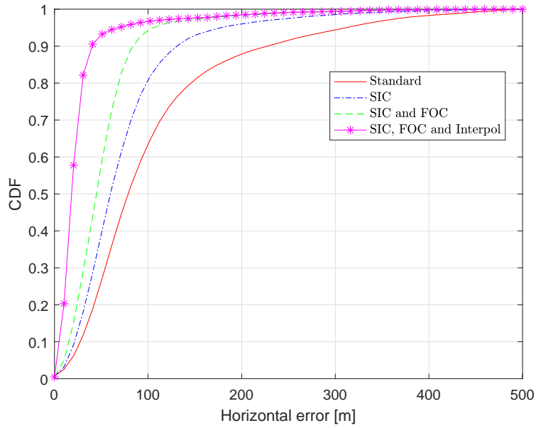
Figure 5.6: Empirical CDF of the horizontal positioning errors in AWGN channel.
