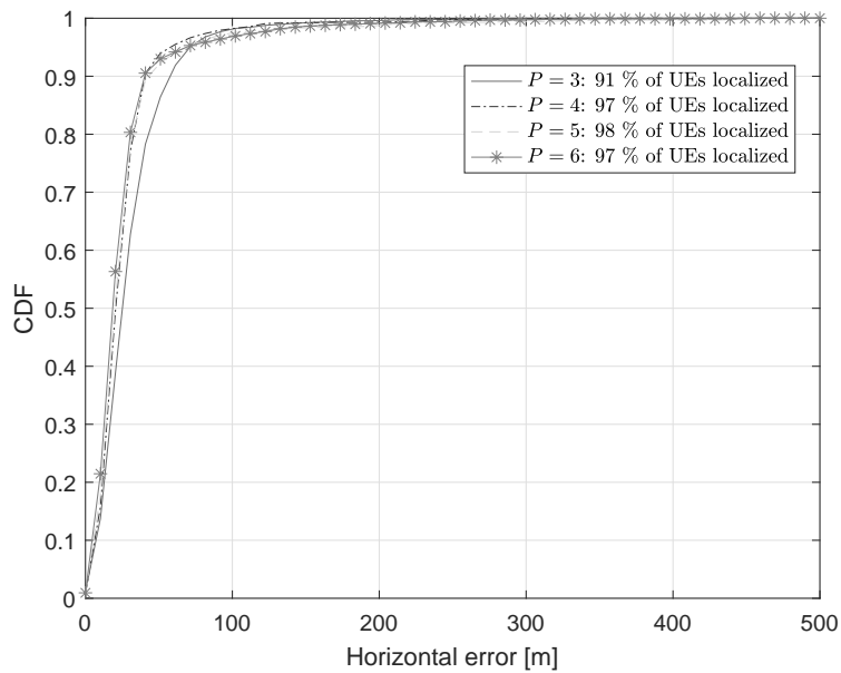
Figure 5.10: Positioning errors and localization ratios for different number of participating eNodeBs P in AWGN channel, using the proposed algorithm with SIC, FOC and interpolation.
