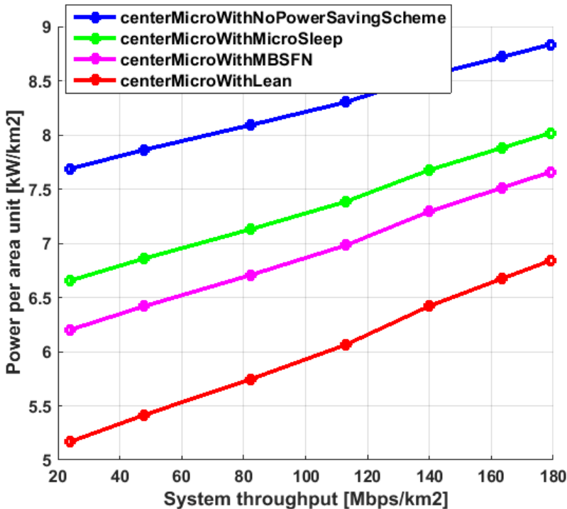
Figure 21. Comparison of Power per area unit versus System throughput for central deployment of micro cells.
