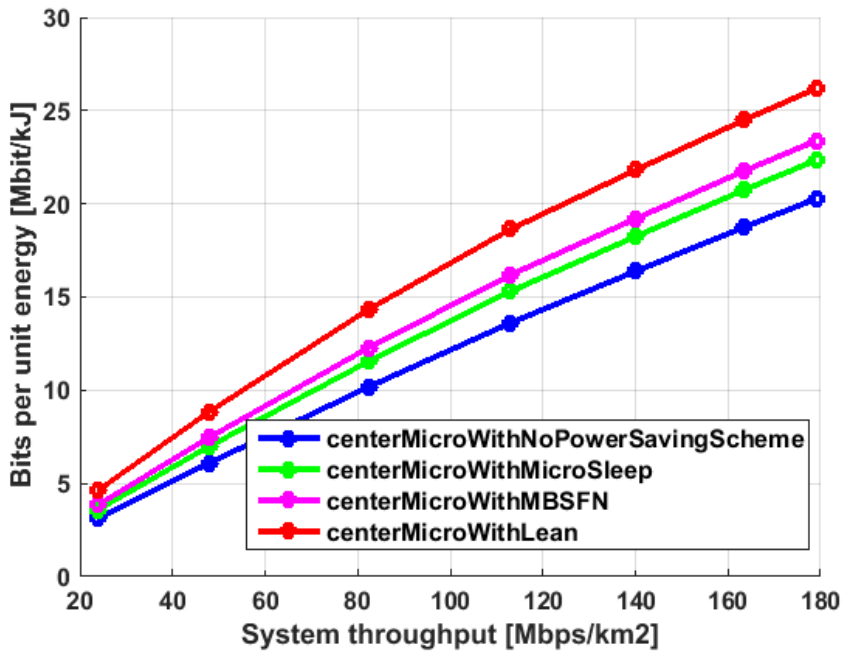
Figure 23. Comparison of bits per unit energy versus system throughput for central deployment of micro cells.
