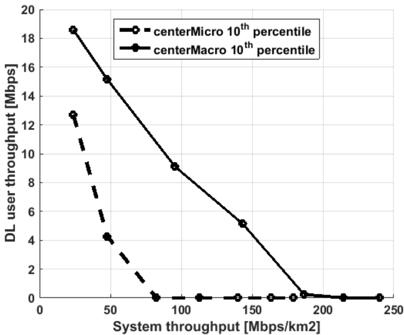
Figure 20. Comparison of DL user throughput for 10th percentile versus system throughput.
