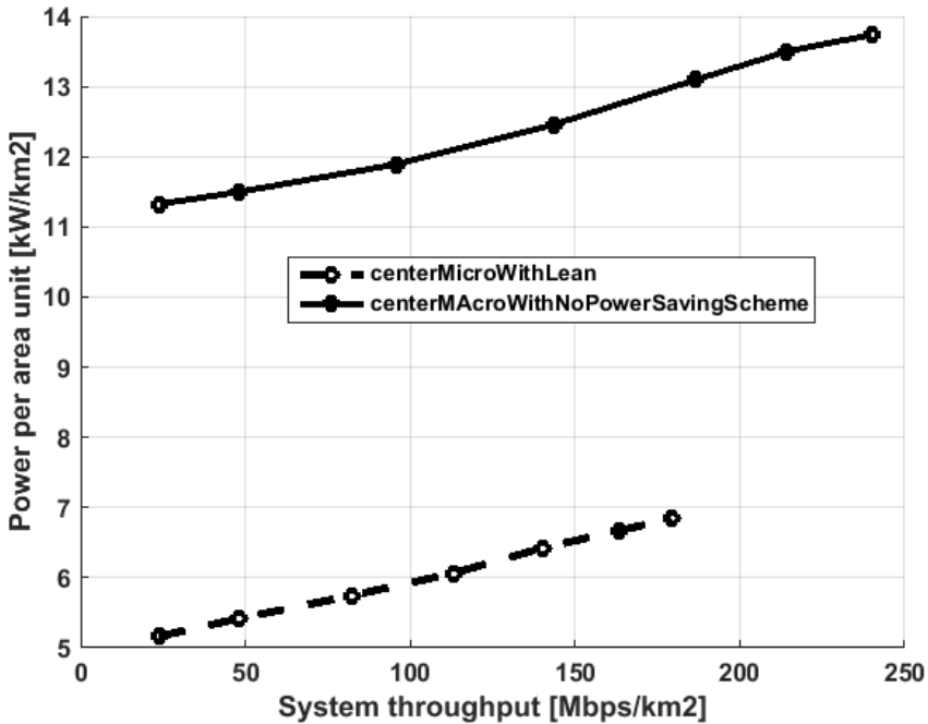
Figure 27. Comparison of Power per area unit versus System throughput for central deployment of macro cells versus micro cells.
