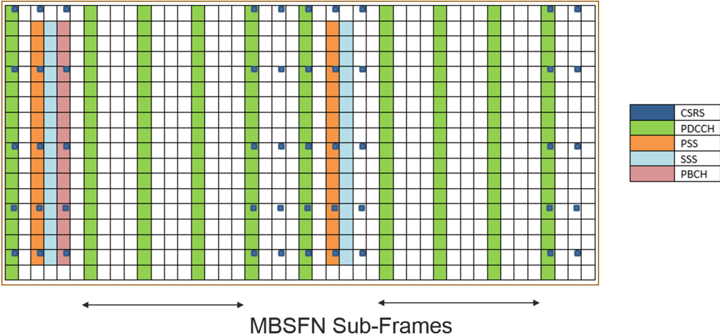
Figure 11. LTE radio frame with six MBSFN sub-frames.
