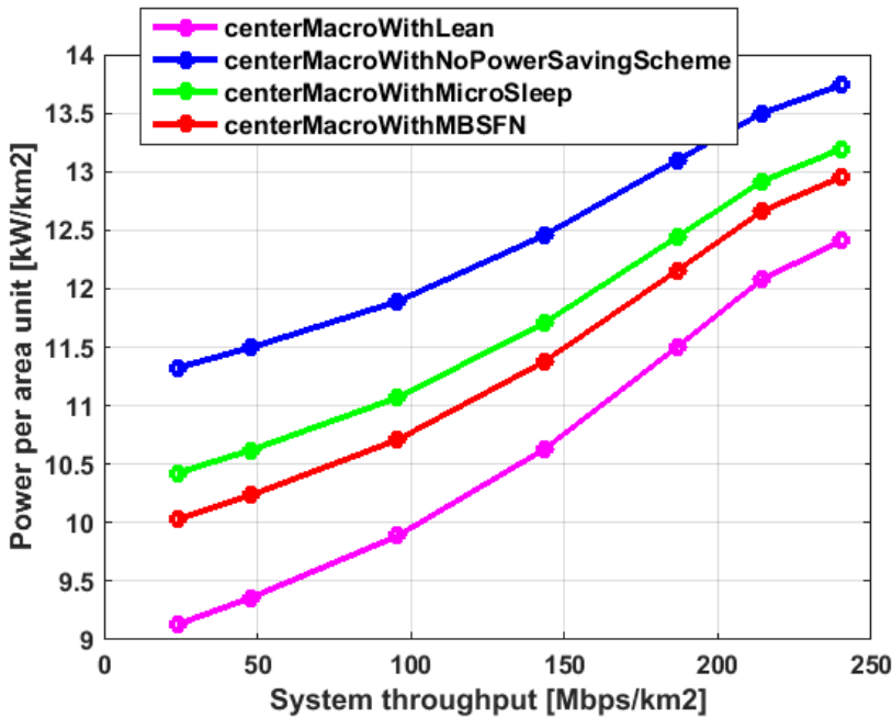
Figure 21. Comparison of power per area unit versus system throughput for central deployment of macro cells.
