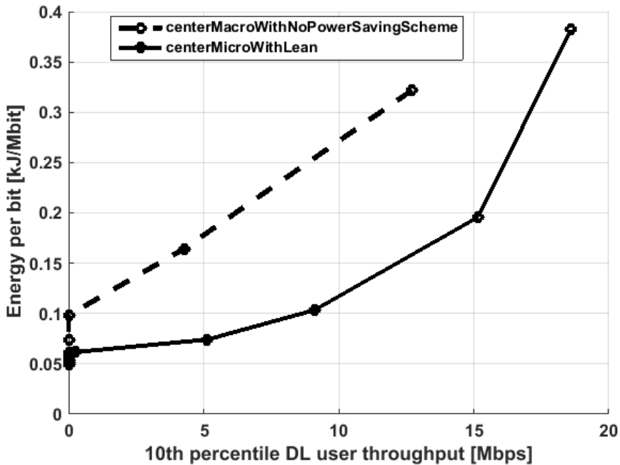
Figure 30. Comparison of energy per bit unit versus system throughput for central deployment of micro cells versus macro cells.
