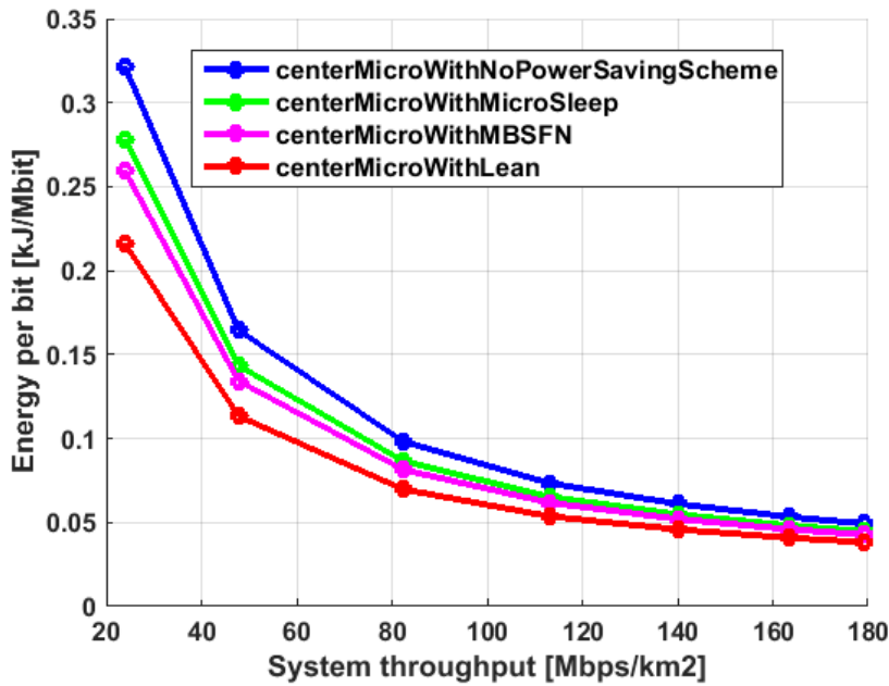
Figure 25. Comparison of energy per bit unit versus system throughput for central deployment of micro cells.
