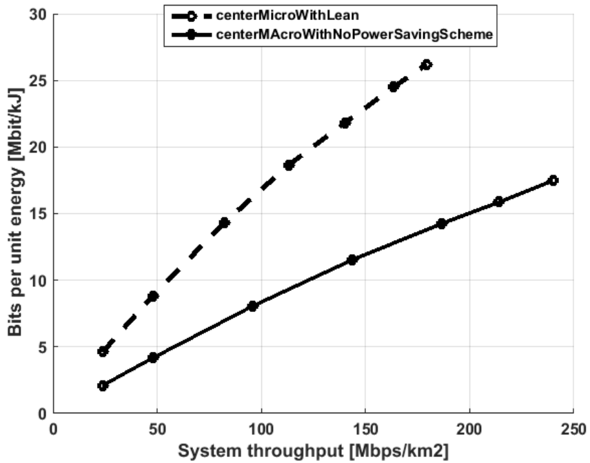
Figure 29. Comparison of bits per unit energy versus system throughput for central deployment of micro cells versus macro cells.
