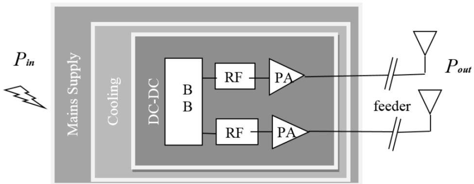
Figure 7. Different components within a base station.
