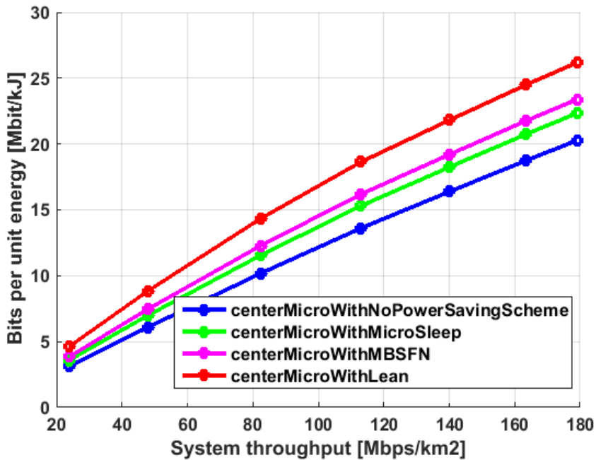
Figure 26. Comparison of bits per unit energy versus system throughput for central deployment of micro cells.
