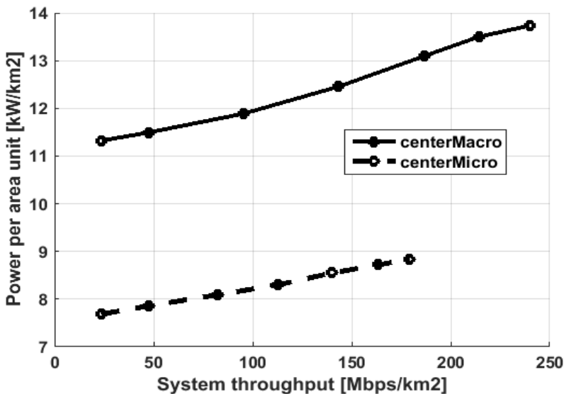
Figure 15. Comparison of Power per area unit versus System throughput for central deployment of macro cells and micro cells.
