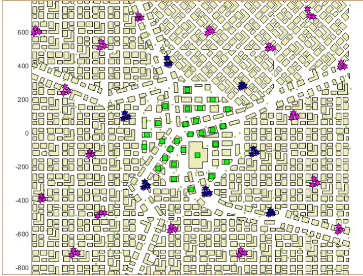
Figure 15. The figure shows deployment of micro cells in the center of the city with macro cells in the surrounding area.
