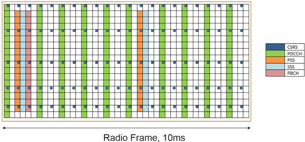
Figure 10. LTE radio frame representation, where PA could be put to sleep when no symbol is being transmitted.
