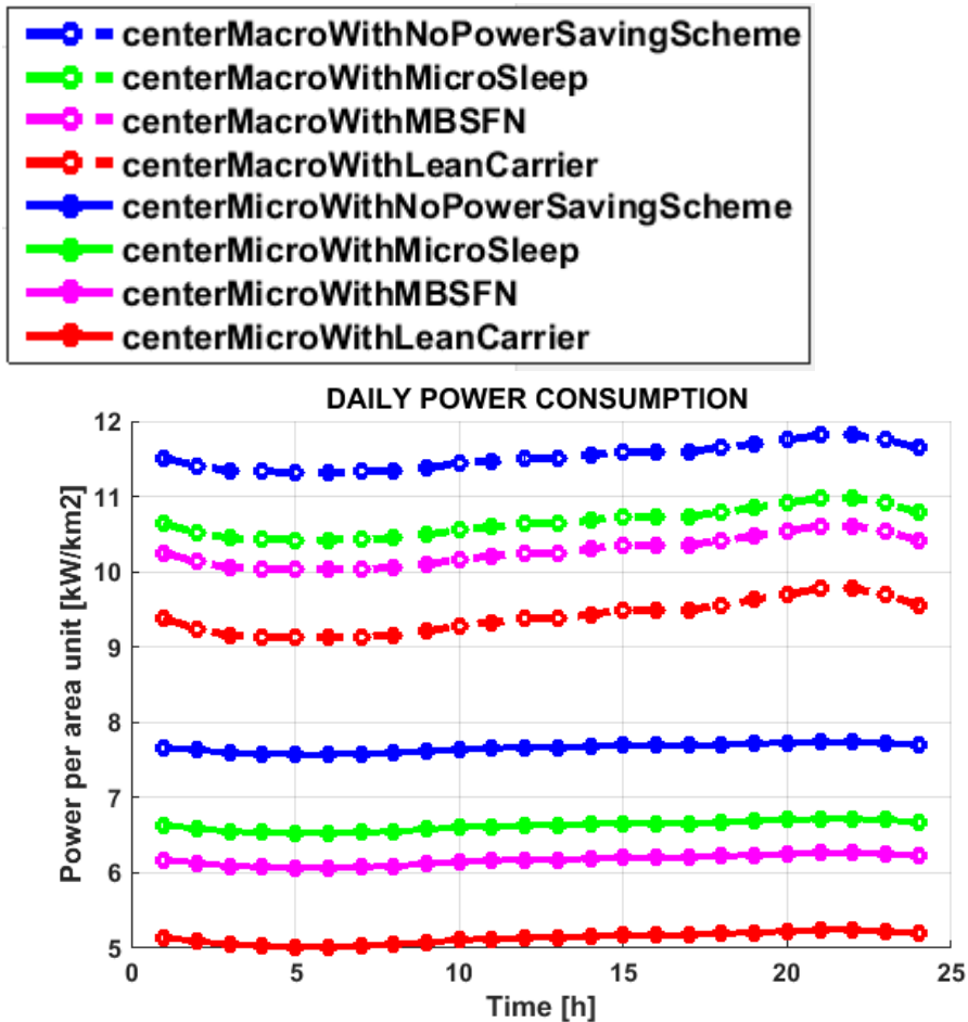
Figure 31. Comparison of daily power consumption in central deployment of micro cells versus macro cells.
