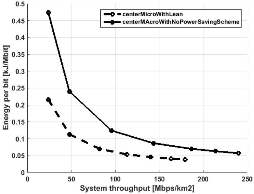
Figure 28. Comparison of energy per bit unit versus system throughput for central deployment of micro cells versus macro cells.
