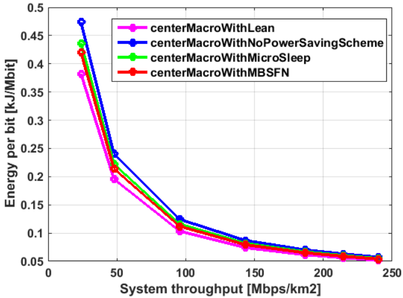
Figure 22. Comparison of energy per bit unit versus system throughput for central deployment of macro cells.
