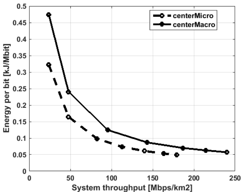
Figure 15. Comparison of Energy per bit versus System throughput for central deployment of macro cells and micro cells.
