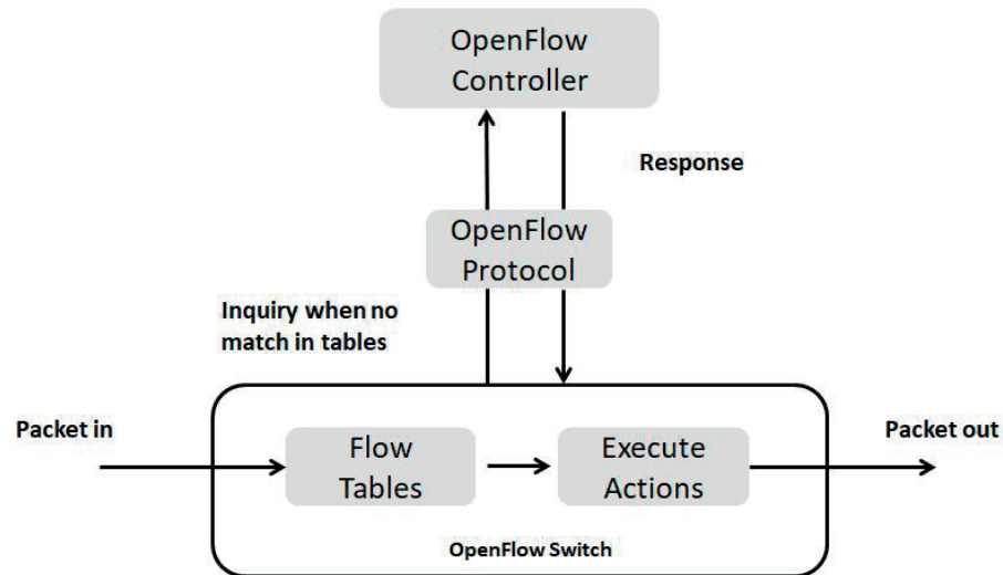
Figure 2.4: OpenFlow Architecture
