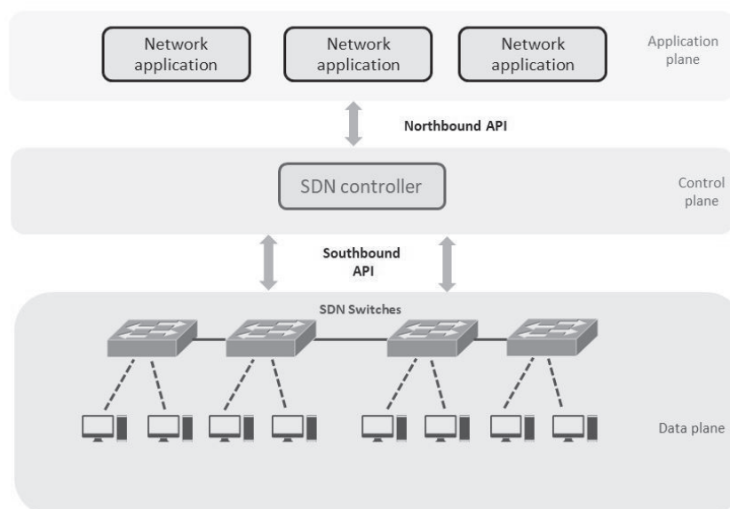
Figure 2.3: SDN architecture
