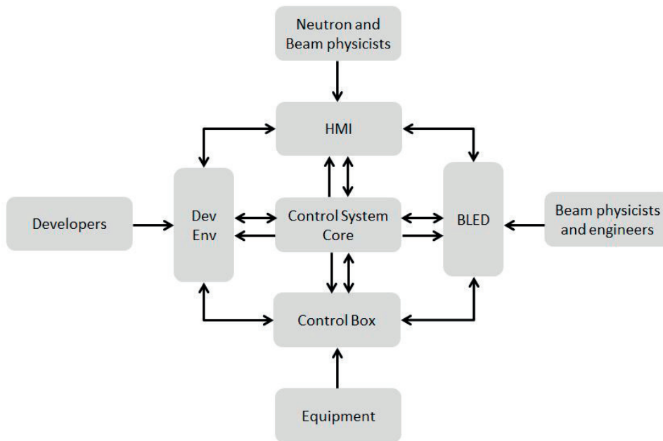
Figure 2.5: Control System Architecture
