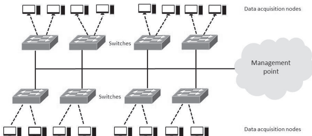
Figure 0.1: Normal production mode
