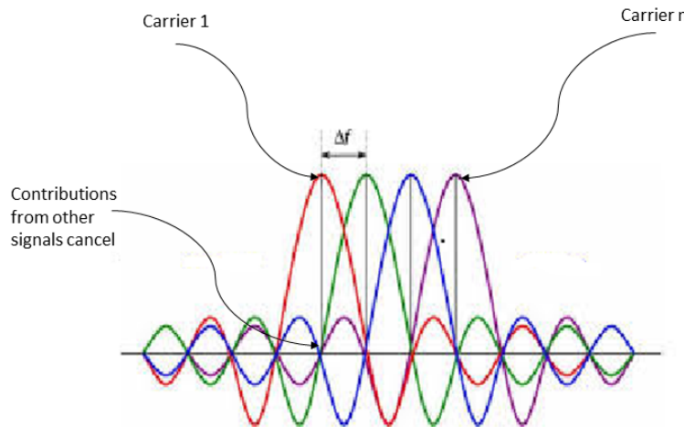
Figure 3.6: OFDM- orthogonality.
