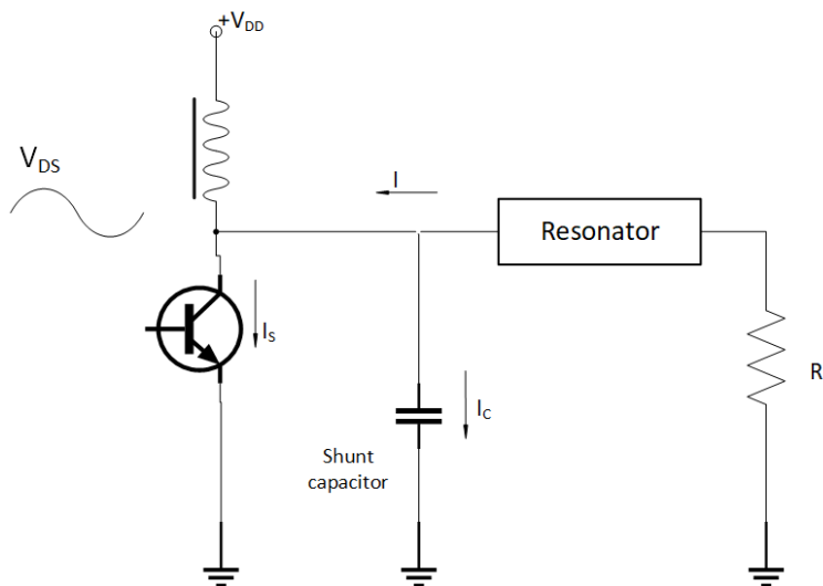
Figure 2.2: High efficiency PA used in PANAMA
