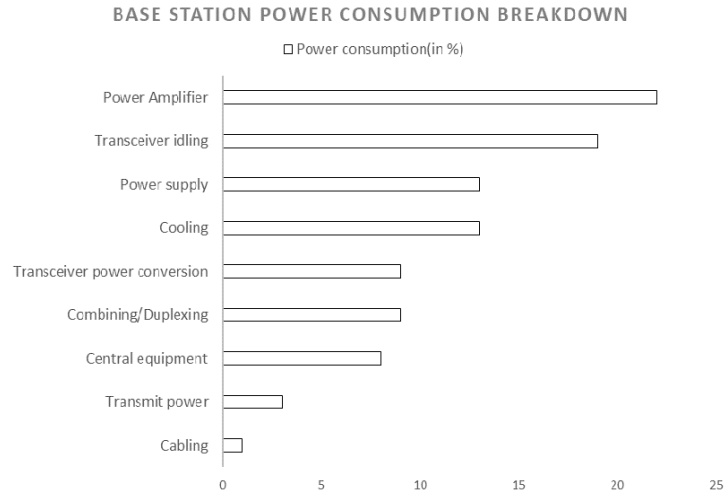
Figure 1.2: Base station power consumption breakdown (Globecom 2010, P.Grant and S.Fletcher, MVCE doc.O-GR-0053)
