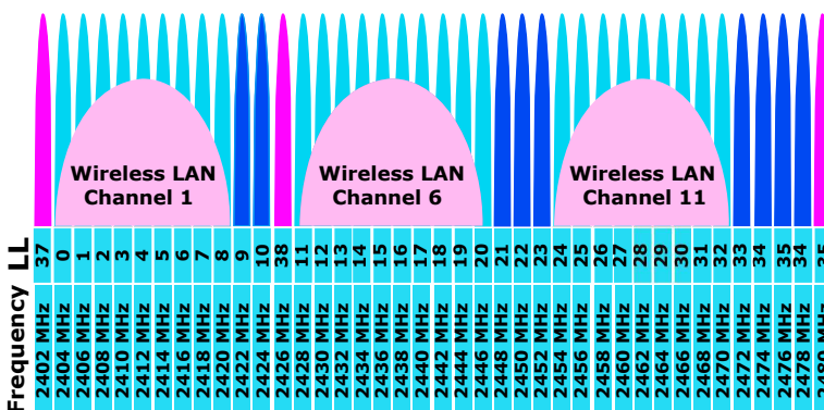
Figure 2.2 BLE channels.
