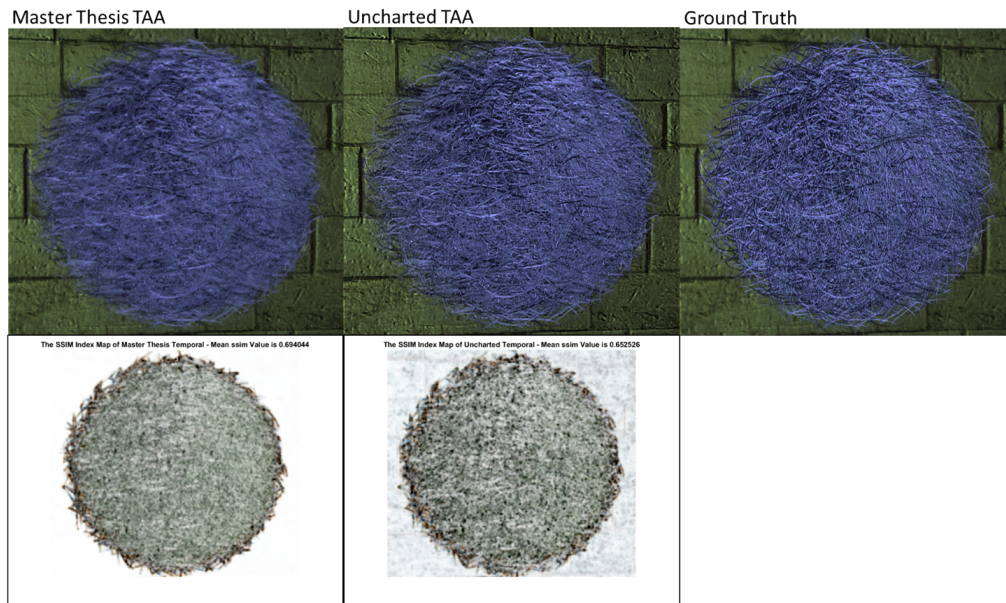
Figure 5.23: Ghosting comparison between Master Thesis TAA, Uncharted TAA and Ground Truth on Test Number 83.
