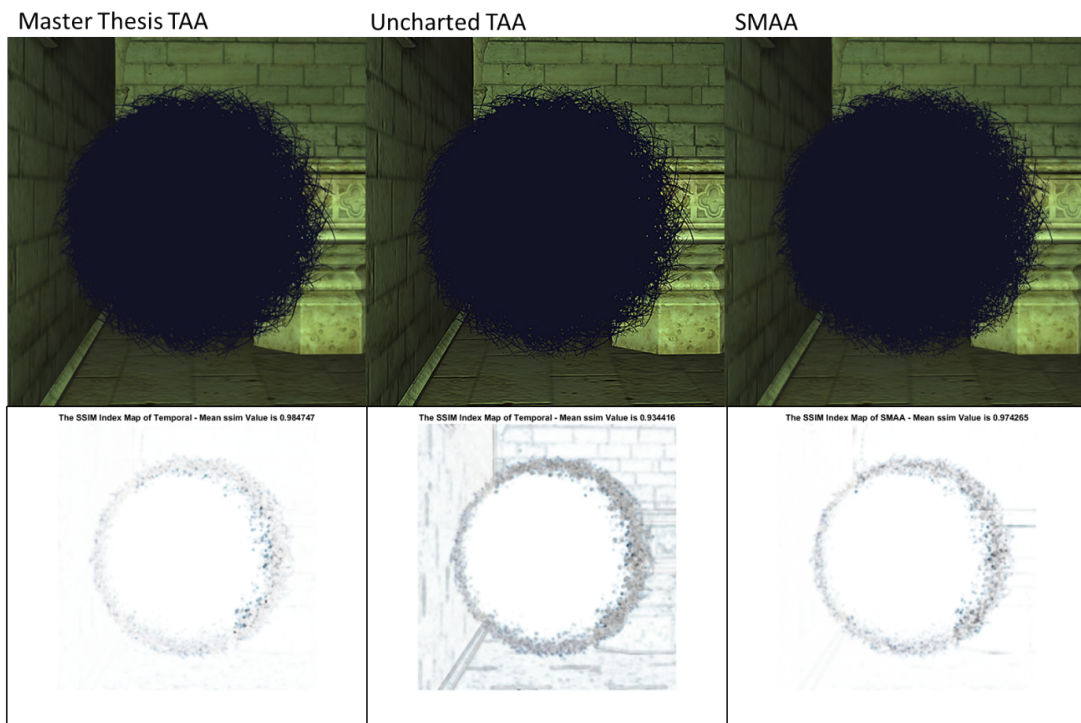
Figure 5.18: Hairball Static Shadow comparison between Master Thesis TAA, Uncharted TAA, and SMAA.
