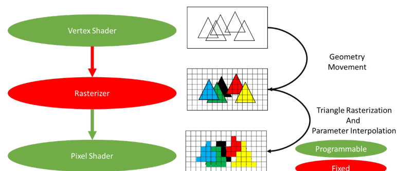
Figure 3.1: Rendering Pipeline, based on EDAF80 5th Lecture. [12]
