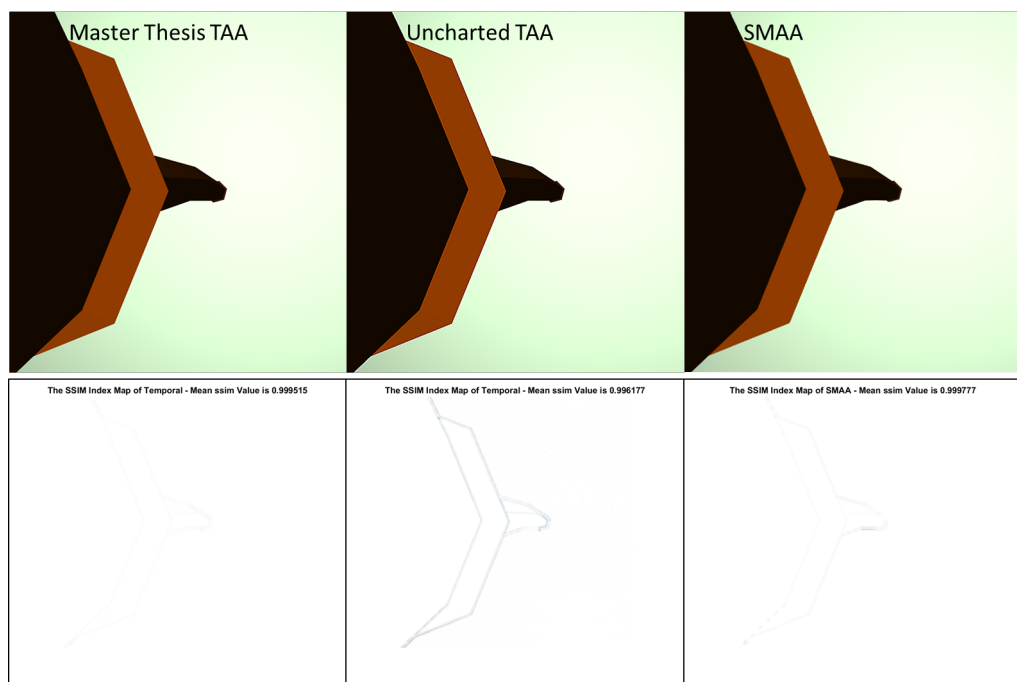
Figure 5.3: Pipe Regular comparison between Master Thesis TAA, Uncharted TAA, and SMAA.
