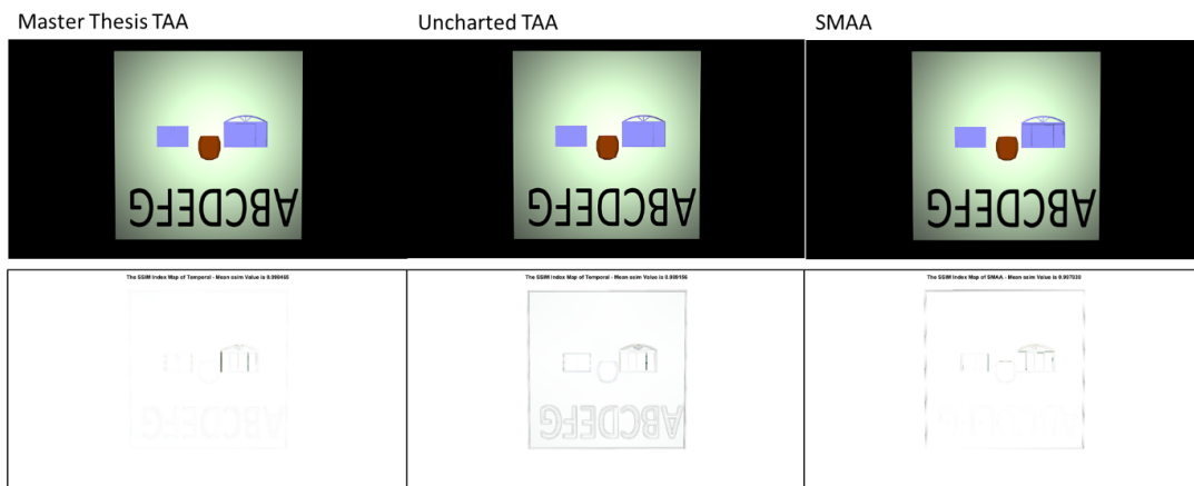
Figure 5.15: Hard Edges comparison between Master Thesis TAA, Uncharted TAA, and SMAA.
