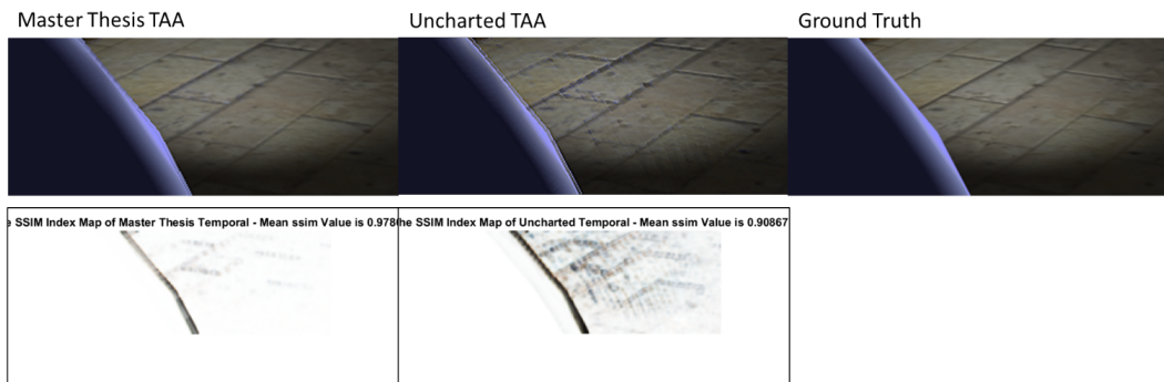
Figure 5.17: Example of Ghosting. Comparison between Master Thesis TAA, Uncharted TAA and Ground Truth on Test Number 19.
