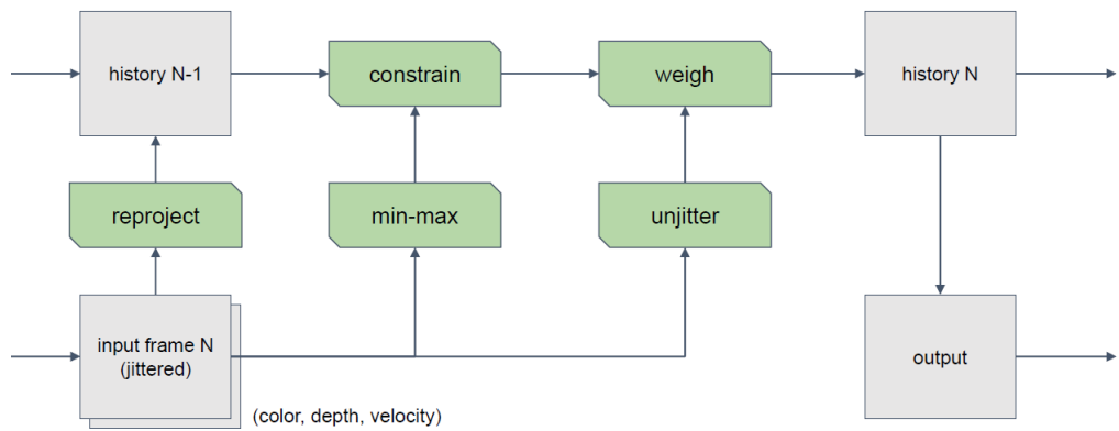
Figure 3.8: Temporal Reprojection Anti-Aliasing process. Image taken from Fuglsand presentation [6]
