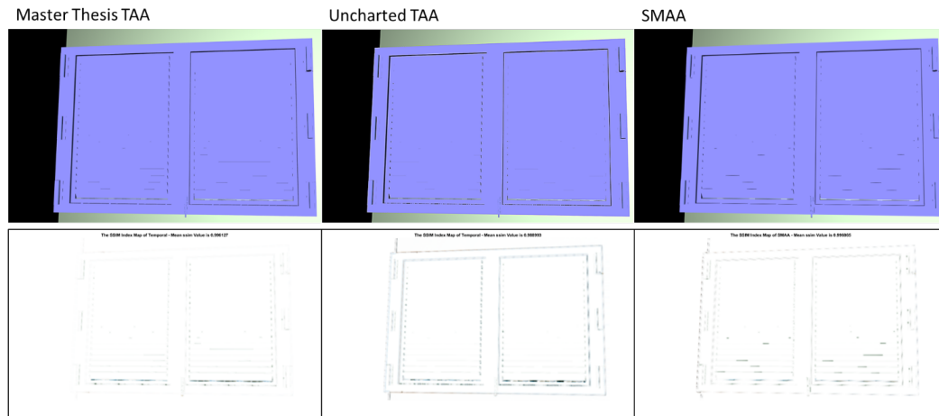
Figure 5.8: Window with Blinds comparison between Master Thesis TAA, Uncharted TAA, and SMAA.
