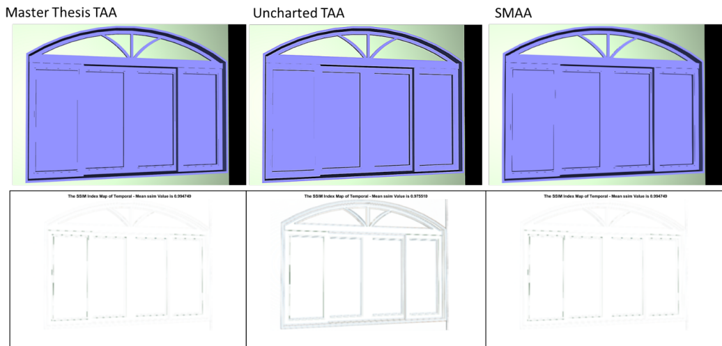
Figure 5.9: Arched Window comparison between Master Thesis TAA, Uncharted TAA, and SMAA.
