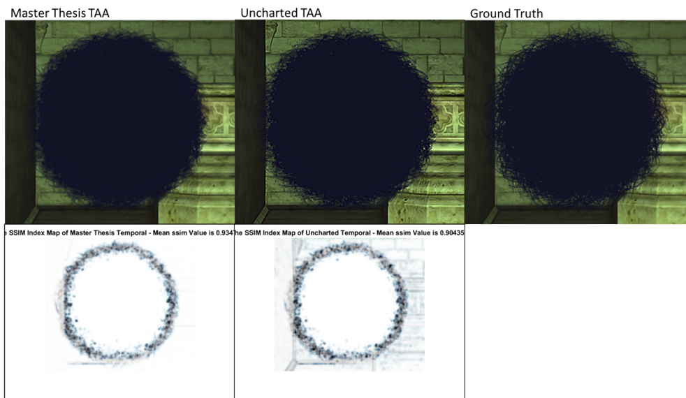
Figure 5.22: Ghosting comparison between Master Thesis TAA, Uncharted TAA and Ground Truth on Test Number 90.
