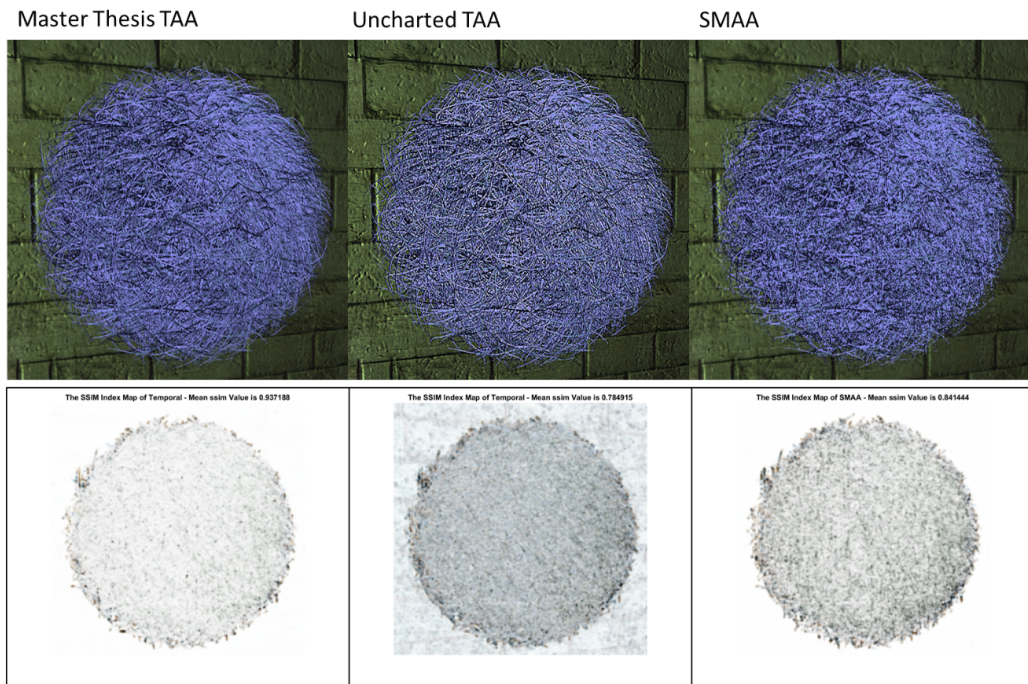
Figure 5.21: Hairball Static Lighted comparison between Master Thesis TAA, Uncharted TAA, and SMAA.
