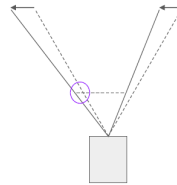
Figure 3.5: Jittering the Projection Process. Image taken from Fuglsand presentation. [6]
