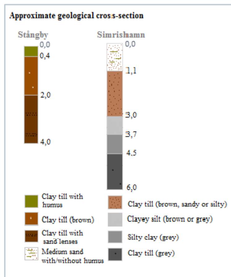
Above: An approximate geological cross-section of both sites (by author, 2018).
