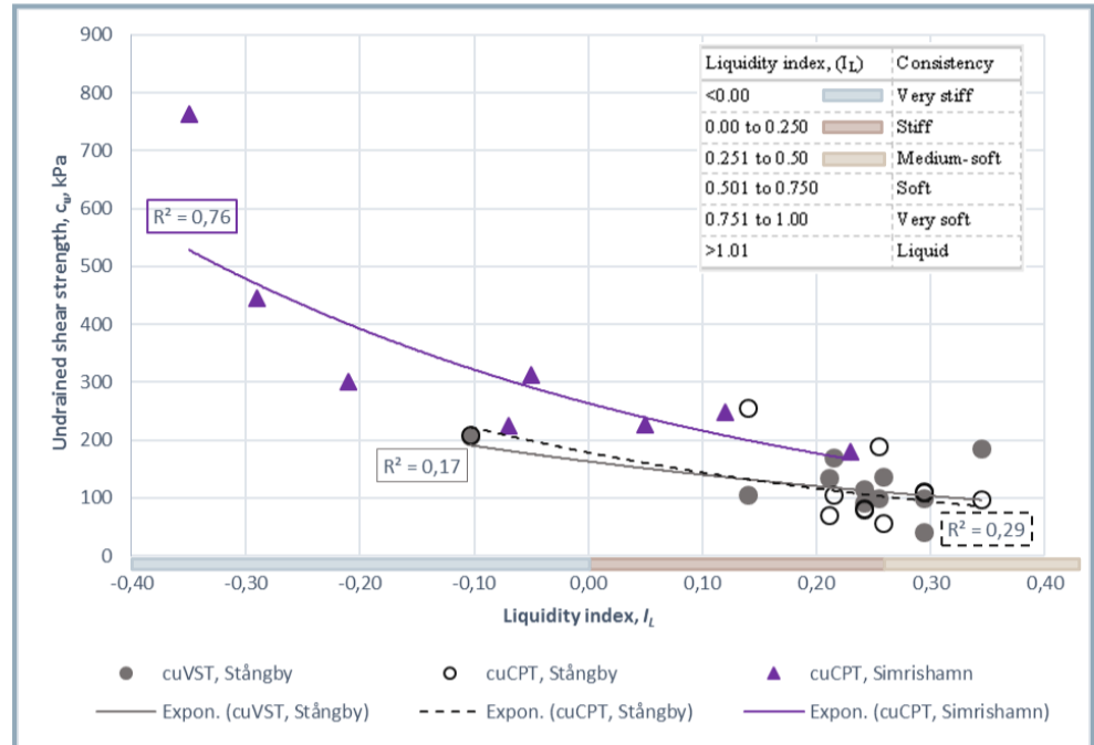
Above: A summary of undrained shear strength and liquidity index from Stångby and Simrishamn sites expressed by the exponential regression lines.
