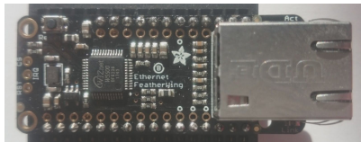
Figur. 3. Ethernet-kort, Ethernet FeatherWing [3]
