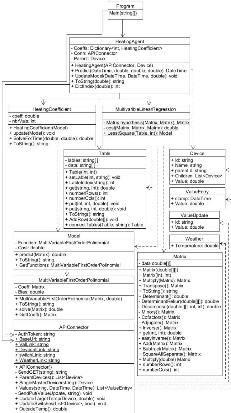
Figure 4.2: Class diagram over the test implementation
