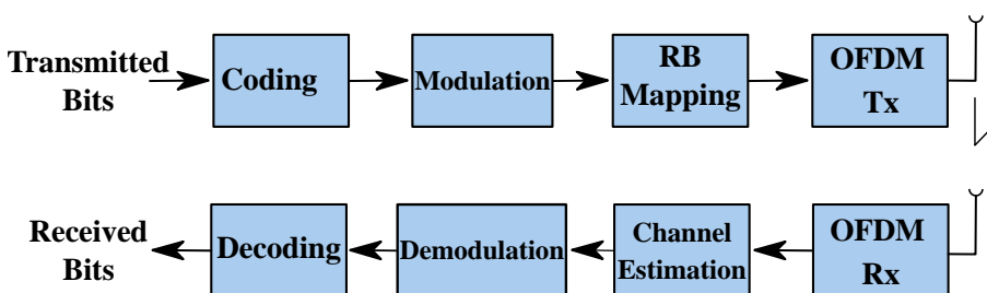
Fig. 5. Block diagram of LTE Transmitter and Receiver
