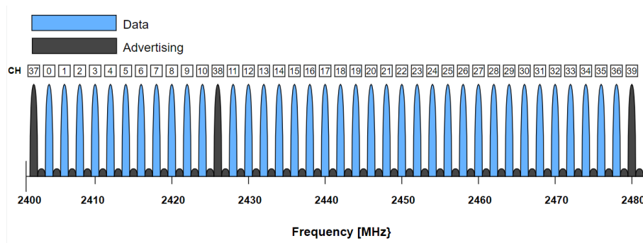
Figure 4.2: BLE channel usage in the ISM band.
